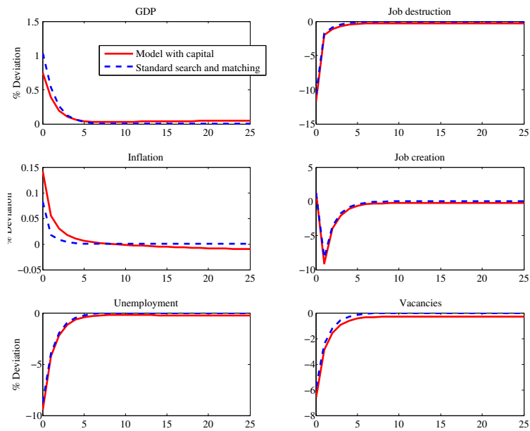
Figure 2: Impulse Responses to a 1 % Interest Rate Shock.
