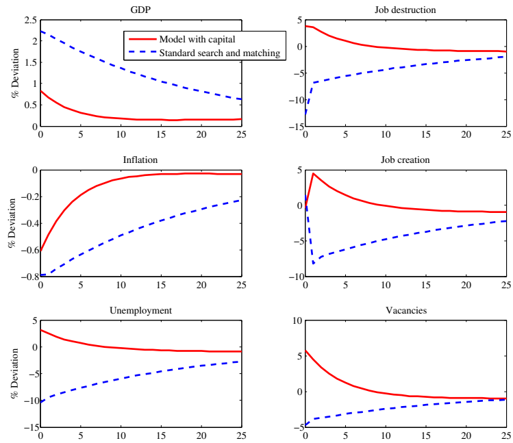
Figure 1: Impulse Responses to a 1 % Productivity Shock.
