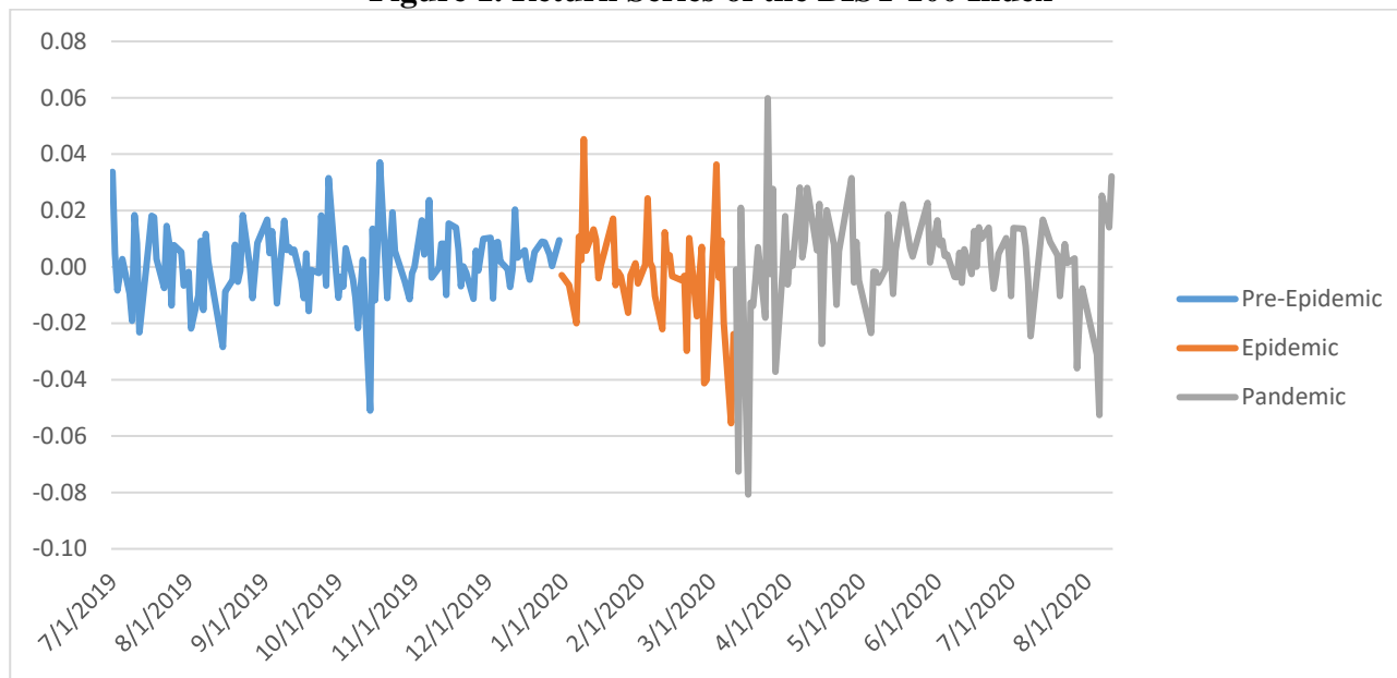
Figure 1. Return Series of the BIST 100 Index
