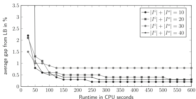
Fig. 3 Average gap of SEQ SJ from lower bound (LB) over time
