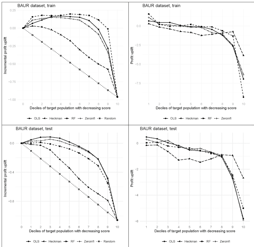
Fig. 3 Application of profit uplift modeling approaches to the BAUR dataset (20 principal components): 50 random subsamples (6/7) of the train set (50%) were used to calibrate the models and predict the profit uplift in the test set (50%). The resulting profit Qini curves (left) and mean profit uplifts (right) were averaged
