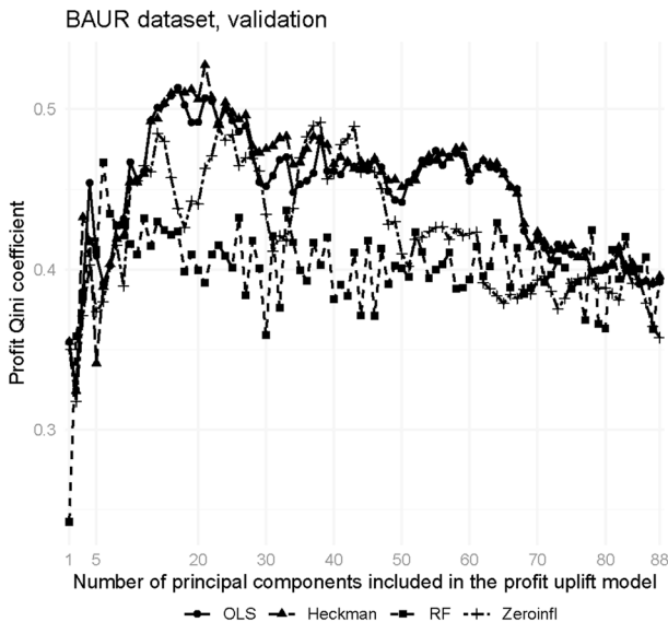
Fig. 2 Profit Qini coefficients for the validation set (3/7 of the BAUR train set) based on training the profit uplift modeling approaches on the calibration set (4/7 of the BAUR train set)
