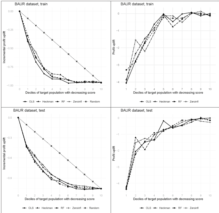
Fig. 6 Application of profit response modeling approaches to the BAUR dataset (20 principal components): 50 random subsamples (6/7) of the train set (50%) were used to calibrate the models and predict the profit uplift in the test set (50%). The resulting profit Qini curves (left) and mean profit uplifts (right) were averaged
