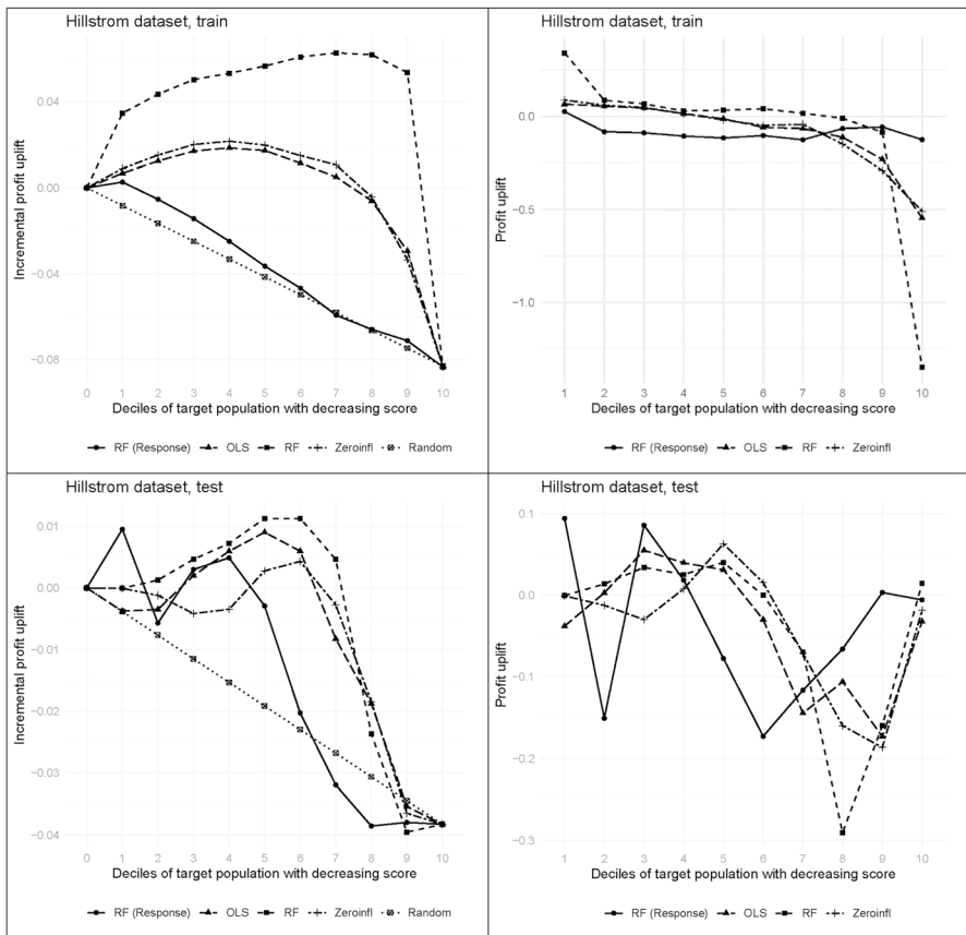
Fig. 7 Results of the application of revenue and profit response and uplift modeling approaches to the Hillstrom dataset: 50 random subsamples (60% of the data) of the train set (70%) were used to calibrate the models and predict the profit uplift in the test set (30%). The resulting Qini curves (left) and mean uplifts (right) were averaged
