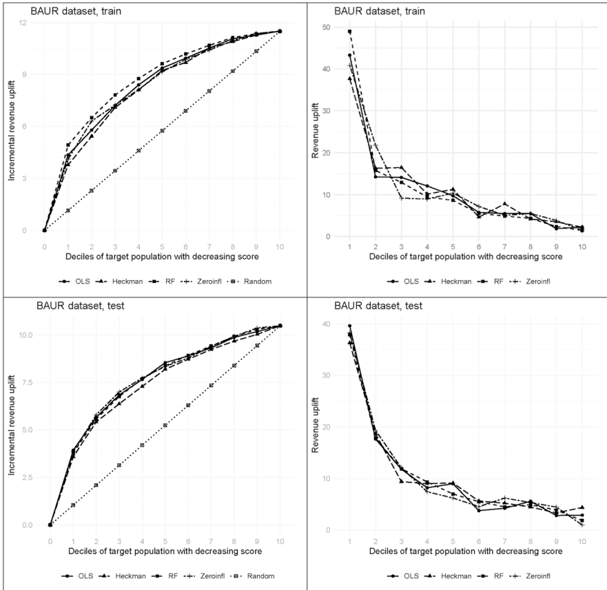
Fig. 4 Application of revenue response modeling approaches to the BAUR dataset (20 principal components): 50 random subsamples (6/7) of the train set (50%) were used to calibrate the models and predict the revenue uplift in the test set (50%). The resulting revenue Qini curves (left) and mean revenue uplifts (right) were averaged
