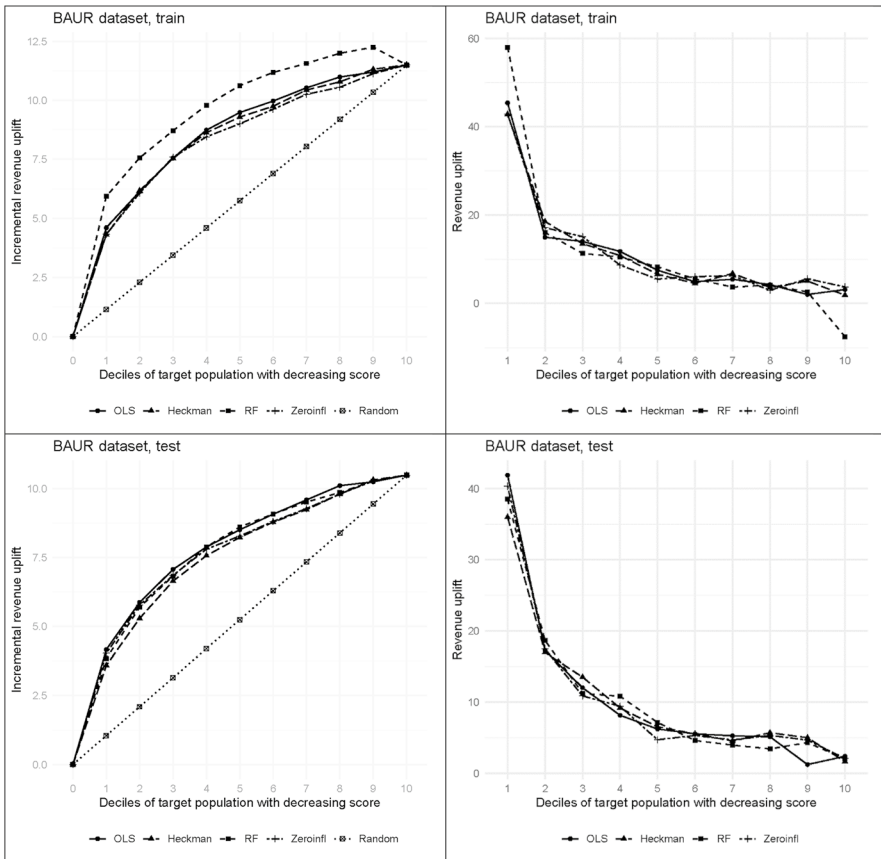
Fig. 5 Application of revenue uplift modeling approaches to the BAUR dataset (20 principal components): 50 random subsamples (6/7) of the train set (50%) were used to calibrate the models and predict the revenue uplift in the test set (50%). The resulting revenue Qini curves (left) and mean revenue uplifts (right) were averaged
