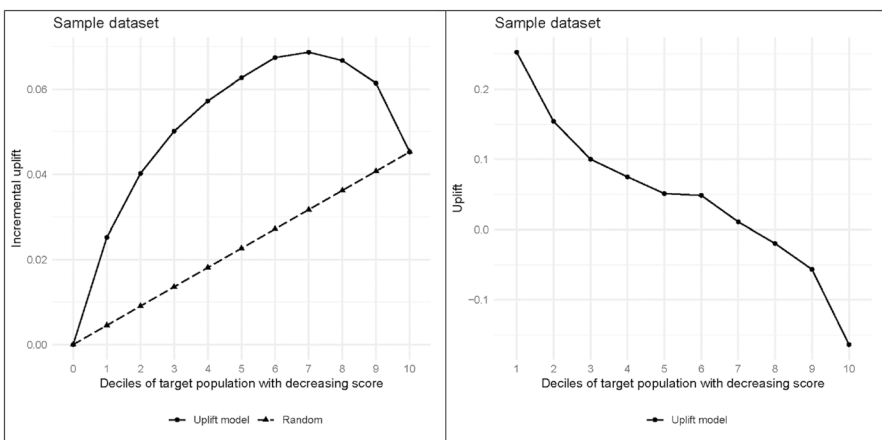
Fig. 1 Qini curve (left) and mean uplifts (right) for a sample dataset. The area between the Qini curve of an uplift model and a random model is the Qini coefficient Q (here: Q=0.0296 ), which can be used for model selection
