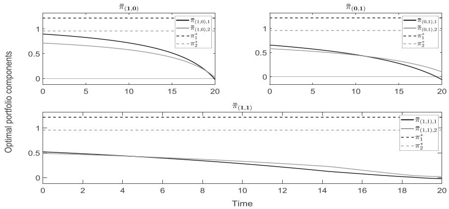
Fig. 7 Two negatively correlated stocks with z^{(1)} = (0.25, 0.15)^T and z^{(2)} = (0.1, 0.1)^T
