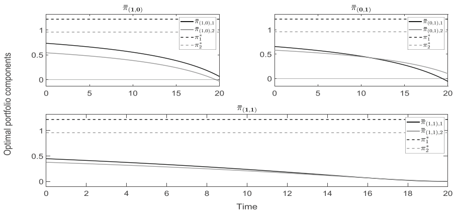
Fig. 4 Two negatively correlated stocks with z^{(1)} = (0.15, 0.25)^T and z^{(2)} = (0.25, 0.15)^T
