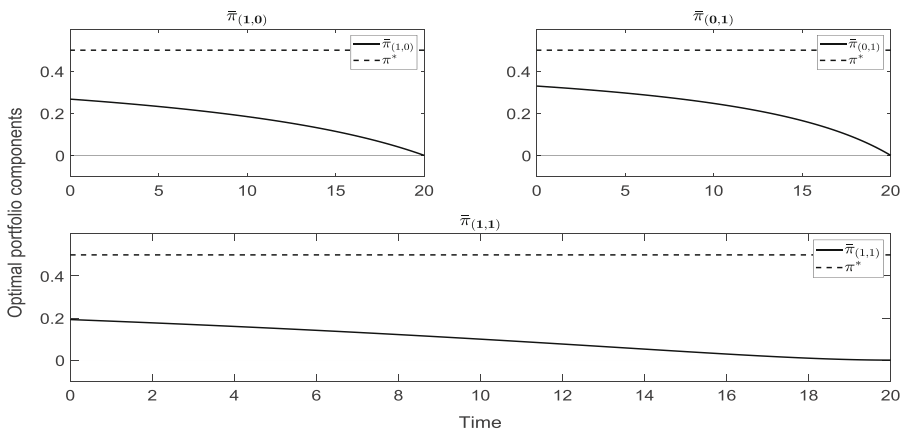
Fig. 1 One stock with z^{(1)} = 0.25 and z^{(2)} = 0.15
