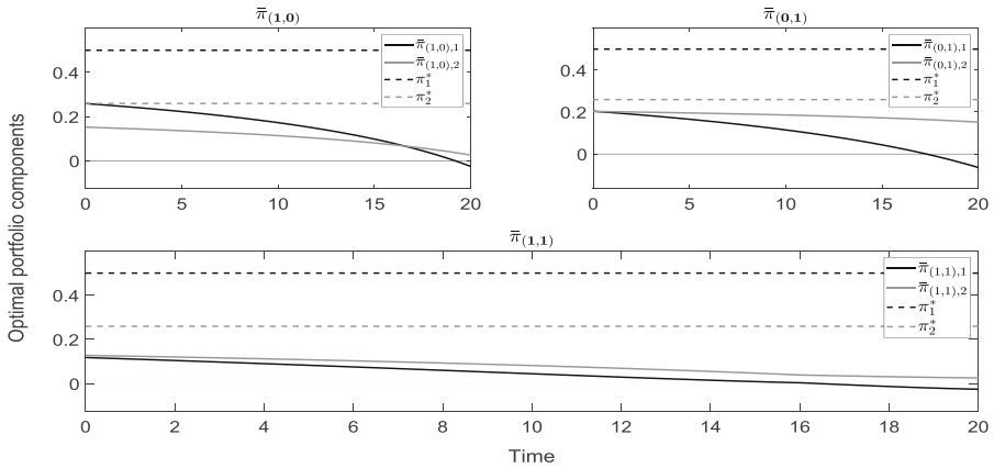
Fig. 3 Two uncorrelated stocks with z^{(1)} = (0.25, 0.25)^T and z^{(2)} = (0.35, 0.15)^T
