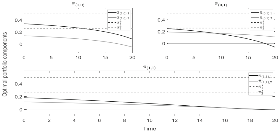
Fig. 2 Two uncorrelated stocks with z^{(1)} = (0.15, 0.25)^T and z^{(2)} = (0.25, 0.15)^T
