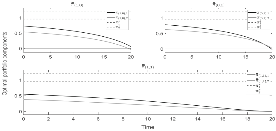
Fig. 5 Two negatively correlated stocks with z^{(1)} = (0.15, 0.25)^T and z^{(2)} = (0.15, 0.15)^T
