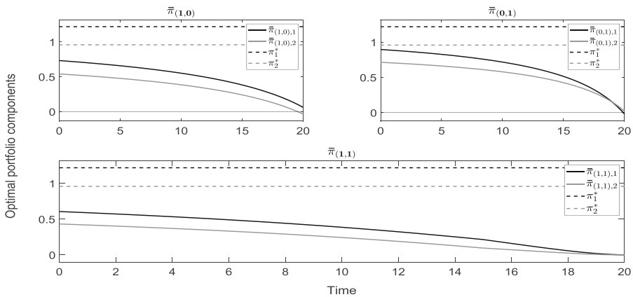
Fig. 6 Two negatively correlated stocks with z^{(1)} = (0.15, 0.25)^T and z^{(2)} = (0.1, 0.1)^T
