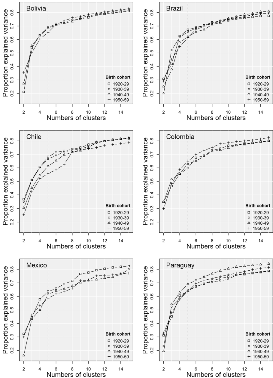
Fig. 7 Proportion of explained variance for several numbers of clusters. Note The proportion of explained variance is computed as the ratio of the sum of squared distances within clusters and the total sum of squared distances according to Studer (2013)
