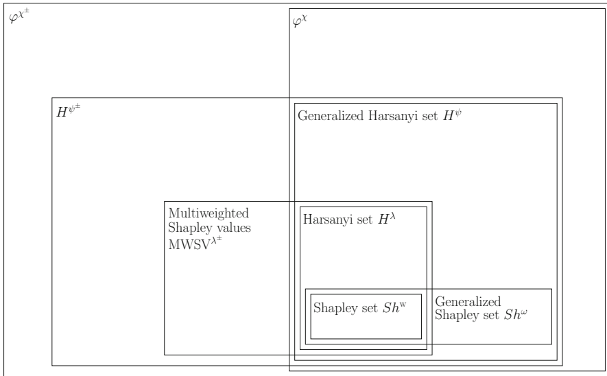
Fig. 1 The subset relationships between some classes of TU-values
