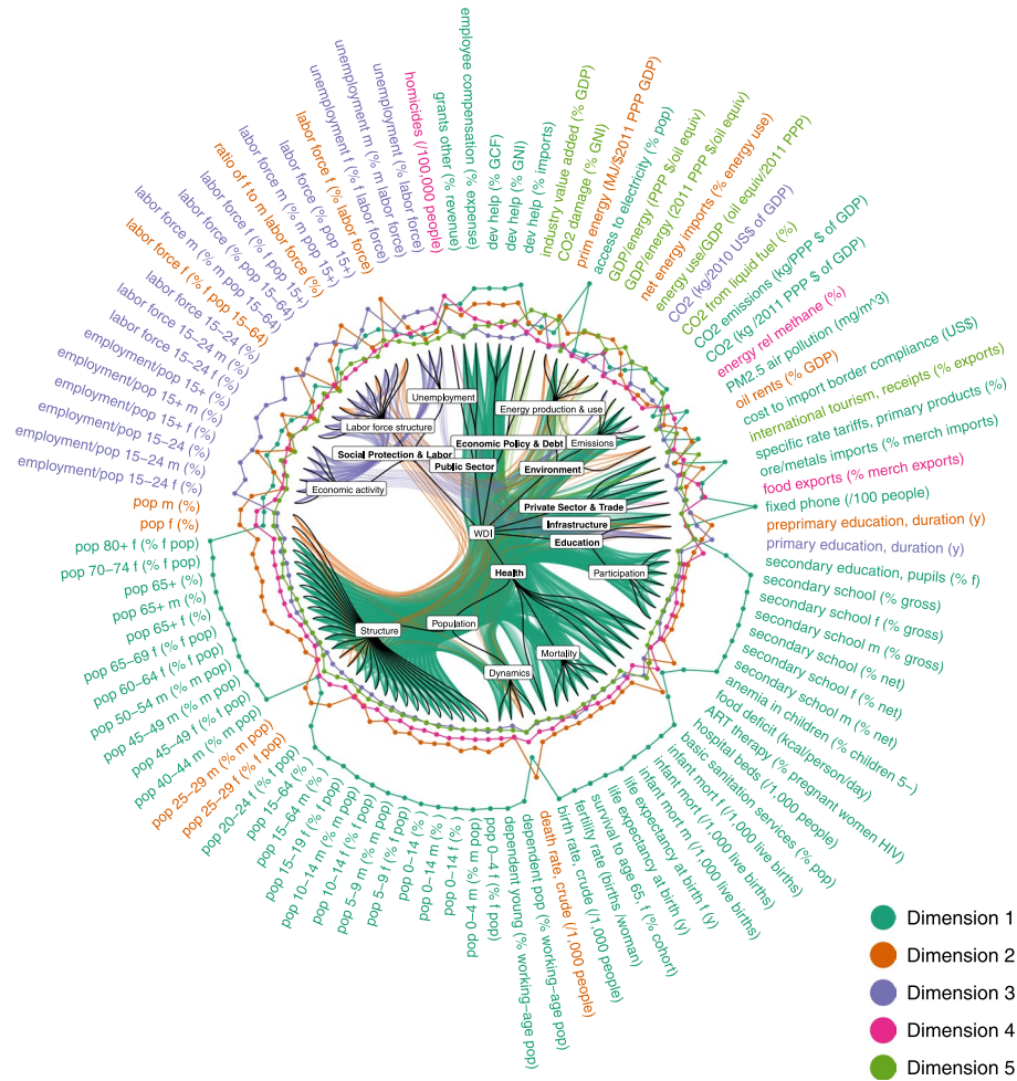
Fig. 4 The importance of single WDIs to the dimensions. Outer circle: indicator names, colored by the maximum distance correlation dimension. Middle circle: distance correlation values with dimensions 1–5. Black center dendrogram: thematic ordering of the indicators by the World Bank. Colored lines in the center circle: connect all indicators that have maximum distance correlation with the same dimension, bundled along the center dendrogram for easier visualization. The figure only shows the WDIs that have the highest distance correlations with dimensions 1–5
