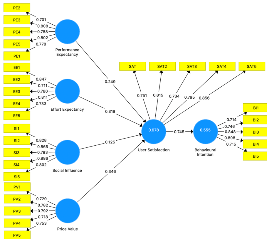
Fig. 2 Result model. Arrows toward the yellow box indicates outer loadings, while arrows pointing on the blue circle represent standardize coefficient effect. R 2 was shown inside the blue circle
