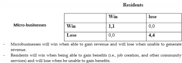
Figure 1. Non-zero game theory.
