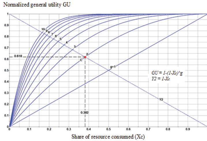
Figure 6. Plots of total utility functions GU(x_c) .
