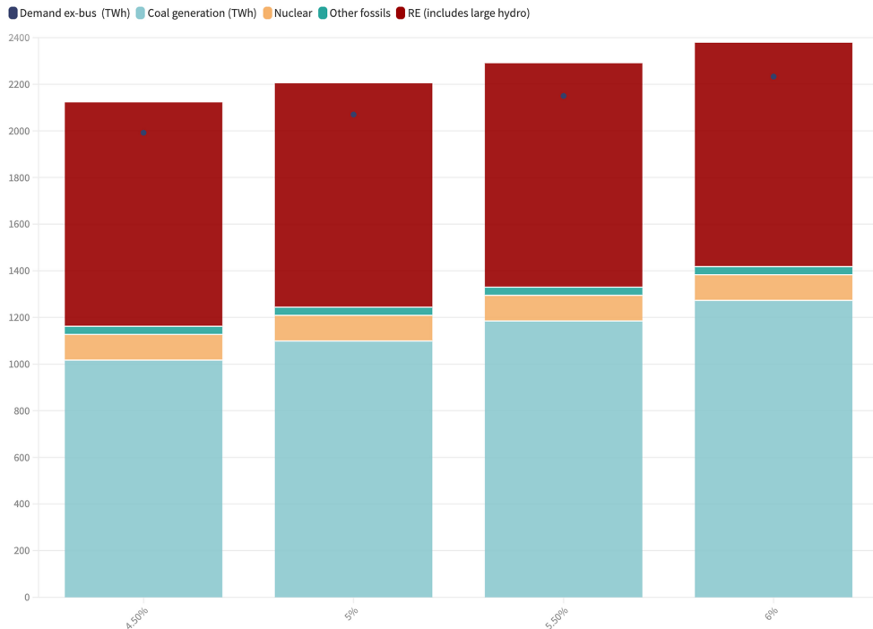
Figure 1.2 Coal-fired generation in FY 2030 under different electricity demand growth scenarios.
