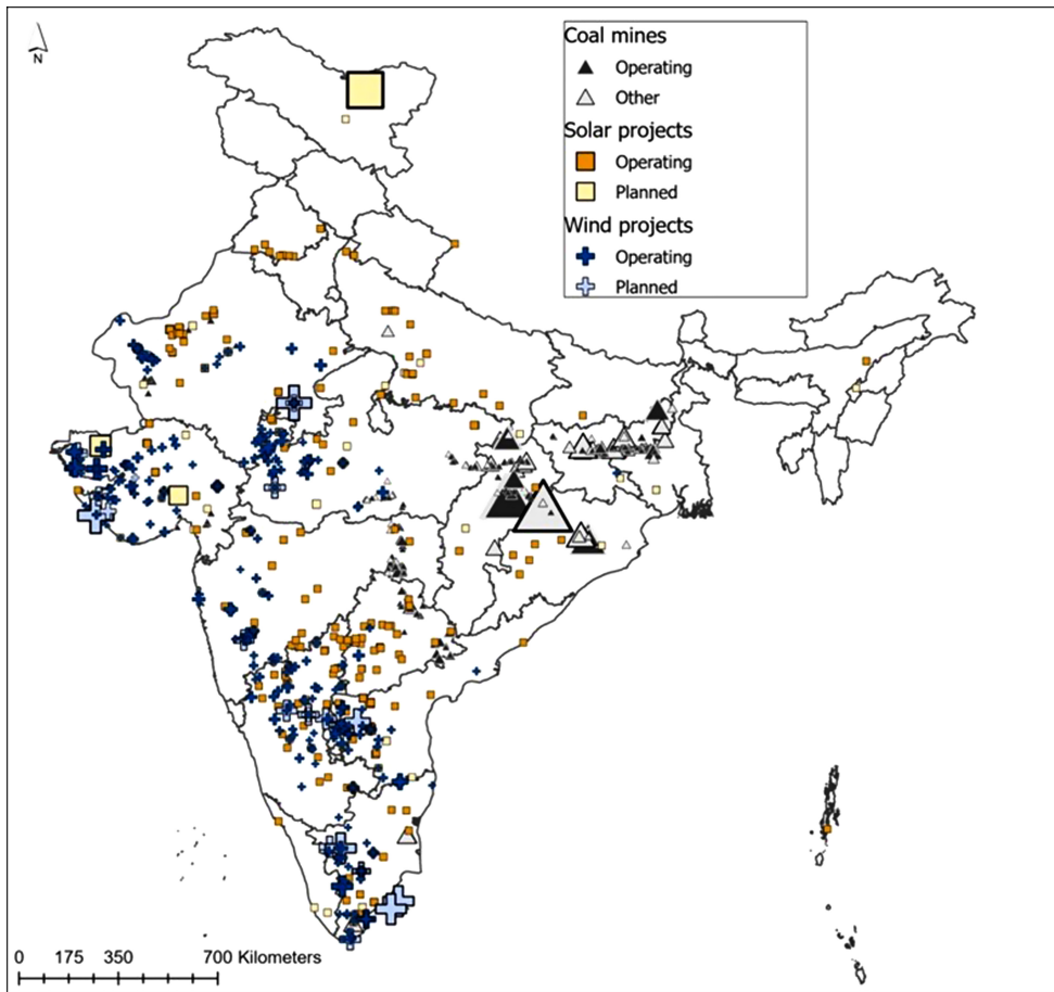
Figure 5.5 Geographical distribution of India's large-scale energy systems (coal, solar, and wind). Global Energy Monitor, 2022
