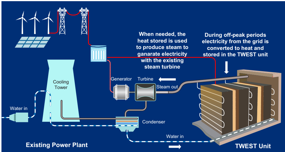
Figure 15.2 Repurposing thermal power plant illustration.
