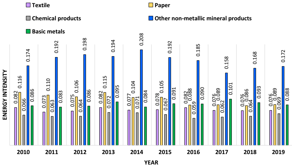
Figure 4.2 Energy intensity trend of five industries from 2010–2019.
