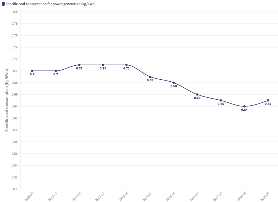
Figure 1.3 Specific coal consumption by coal-based power stations in India.
