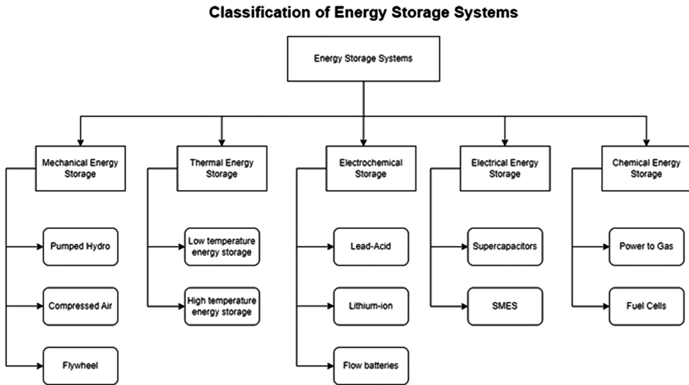
Figure 15.1 Classification of energy storage systems based on the form of energy stored.
