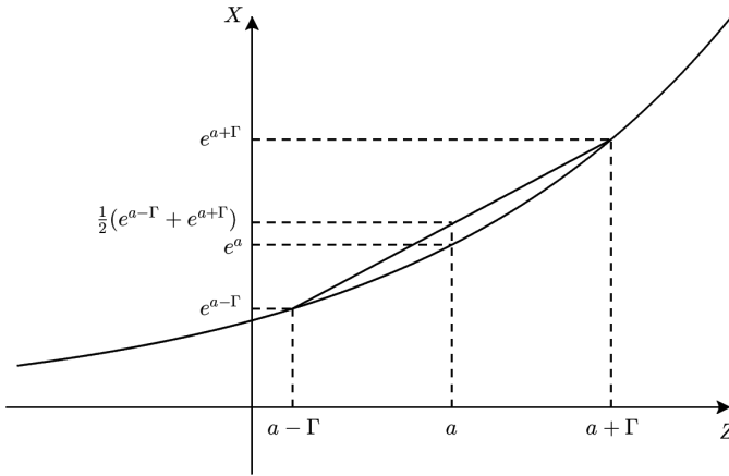
Notes: Figure 1 illustrates values of the log-normally distributed variable X as a function of the normally distributed variable Z according to X = e^Z .
