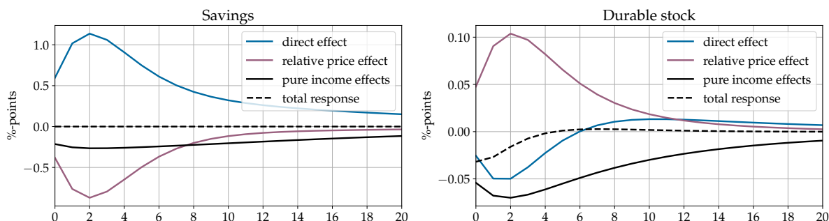
Figure 4: Portfolio-based response decomposition
