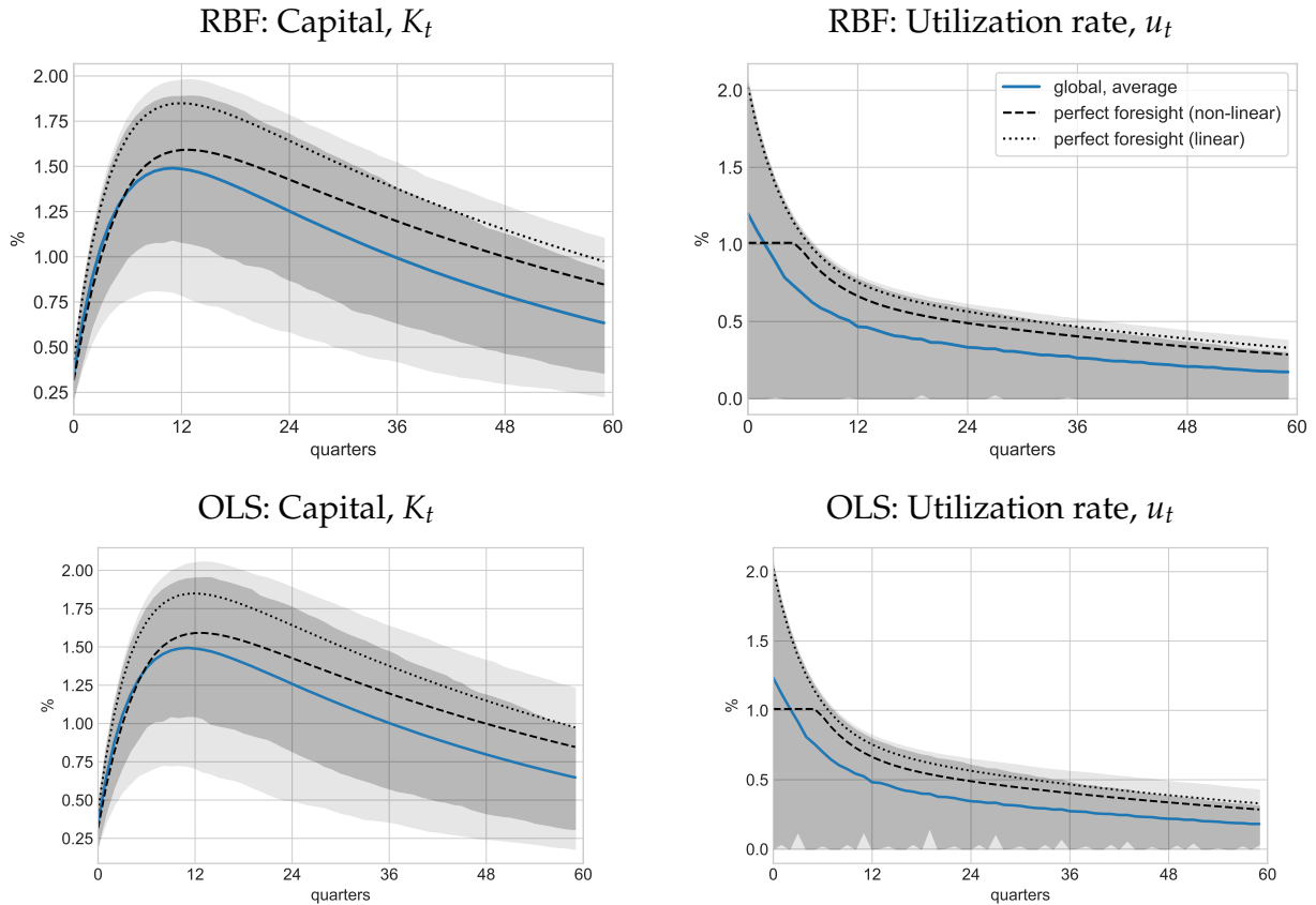
Figure 9: Impulse-responses: State-dependence
