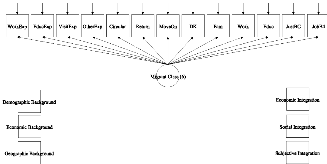
Figure 3: Analytic Strategy
