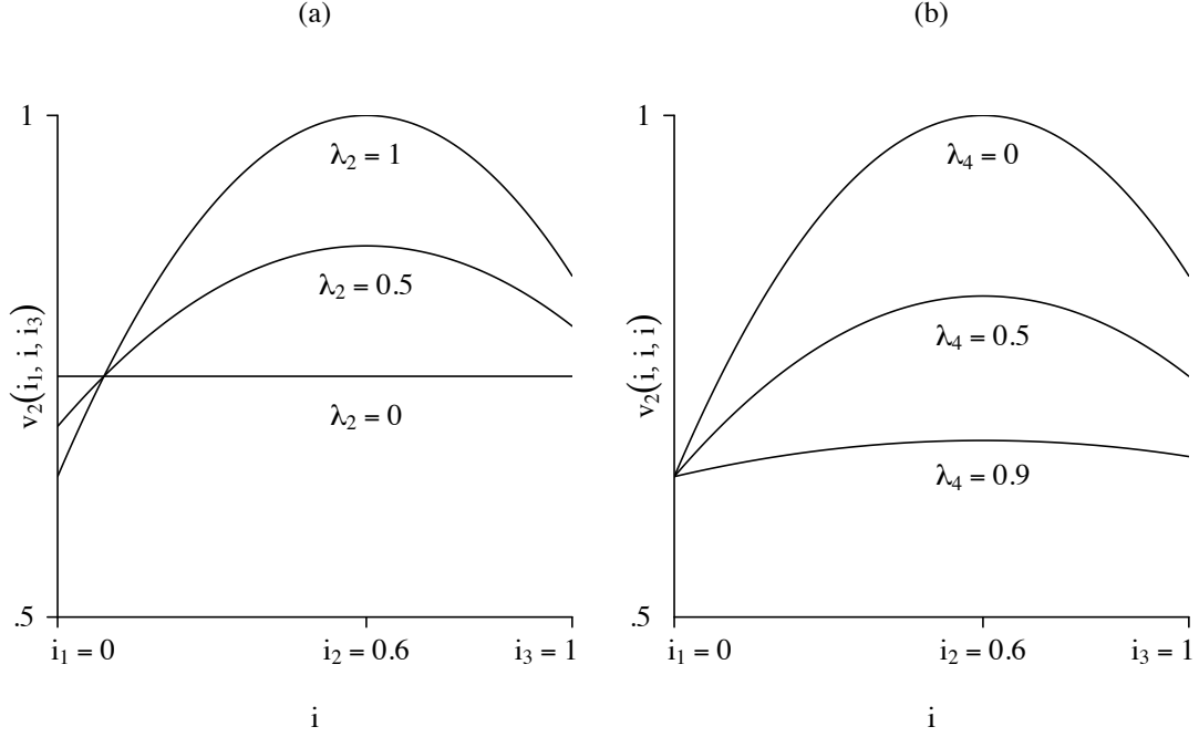
Figure 1: An Illustration of the Indirect Utility Function of Player 2 in Example
