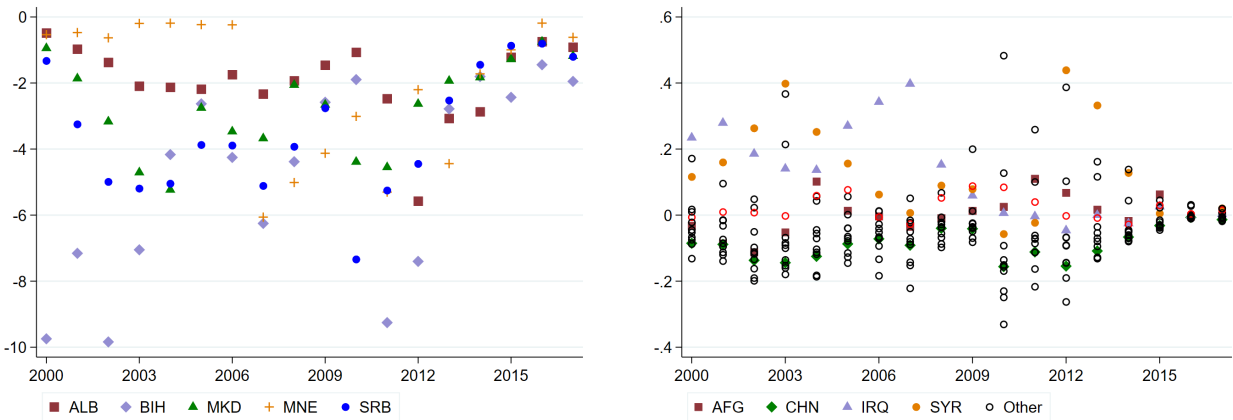
Figure D.4: Variations of the origin-specific multilateral resistance term W_i
