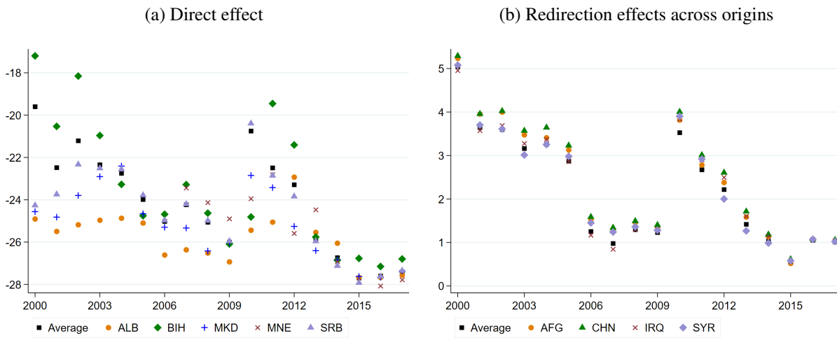
Figure 4: Effect of the counterfactual policy scenario in Sweden
