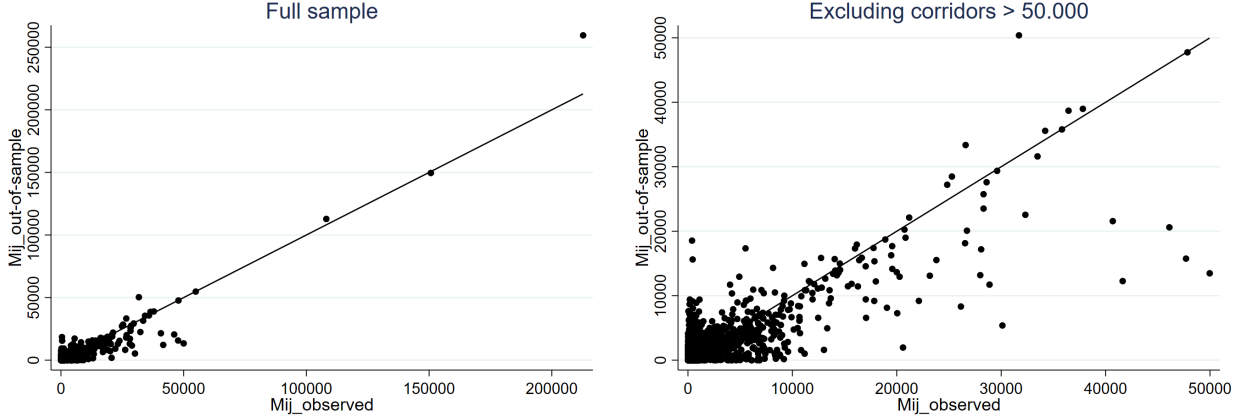
Figure D.1: Out-of-sample calibration of M_{ij} (2000-2009)
