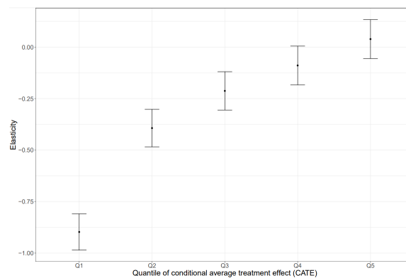
Figure 5: Sorted Group Average Treatment Effects
