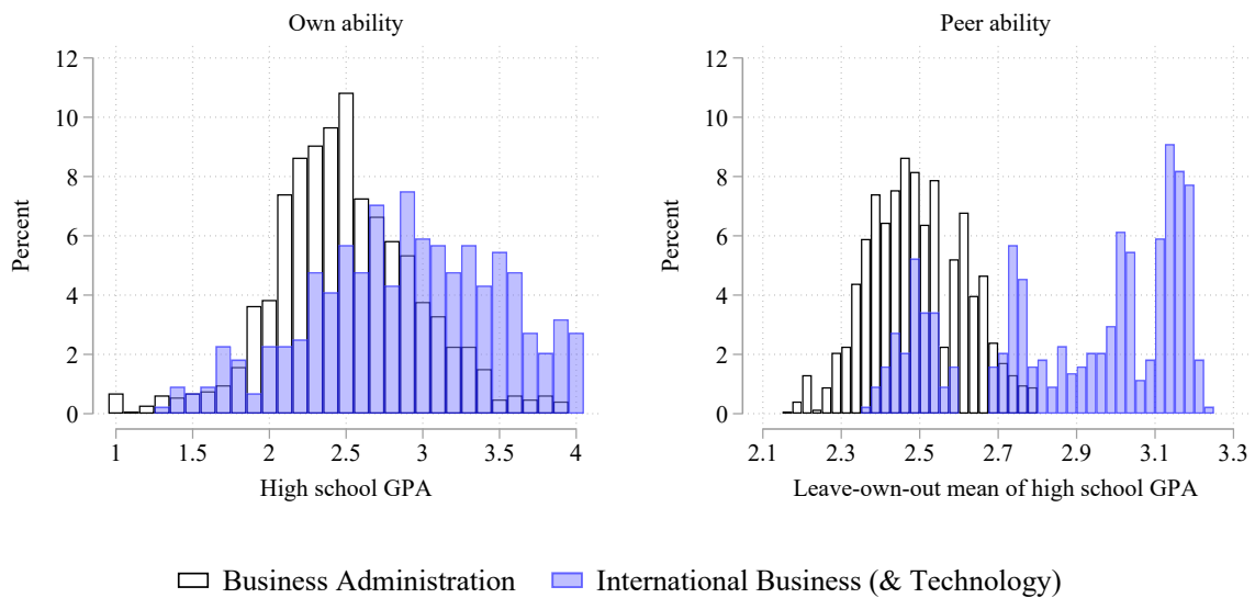
Figure 2: Distribution of ability – by study program
