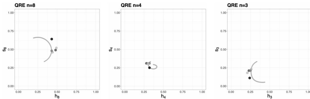
FIGURE 9. Quantal response equilibrium.
