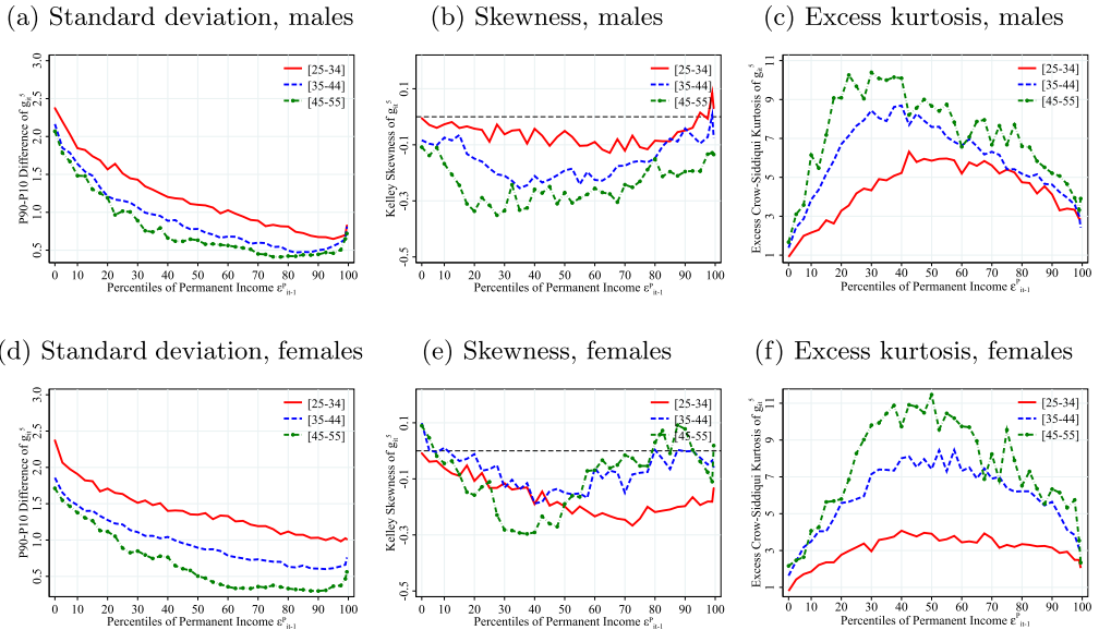
FIGURE A15. Dispersion, skewness, and kurtosis of 5-year earnings changes. Notes: H sample, 5-year changes in residualized log earnings, data pooling 2008–2013. On the x-axis, we report percentiles of residualized log permanent earnings \epsilon_{it}^P . In panels (a) and (d), we show the P90–P10 percentile difference, in panels (b) and (e) we show Kelley skewness, and in panels (c) and (f) we show excess Crow–Siddiqui kurtosis. The various curves on the graphs corresponds to various age groups: between 25 and 34 years, between 35 and 44, and between 45 and 55 years, respectively.
