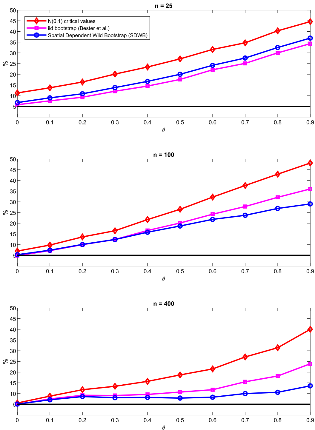
FIGURE 2. Rejection rate with N(0, 2) error in locations.
