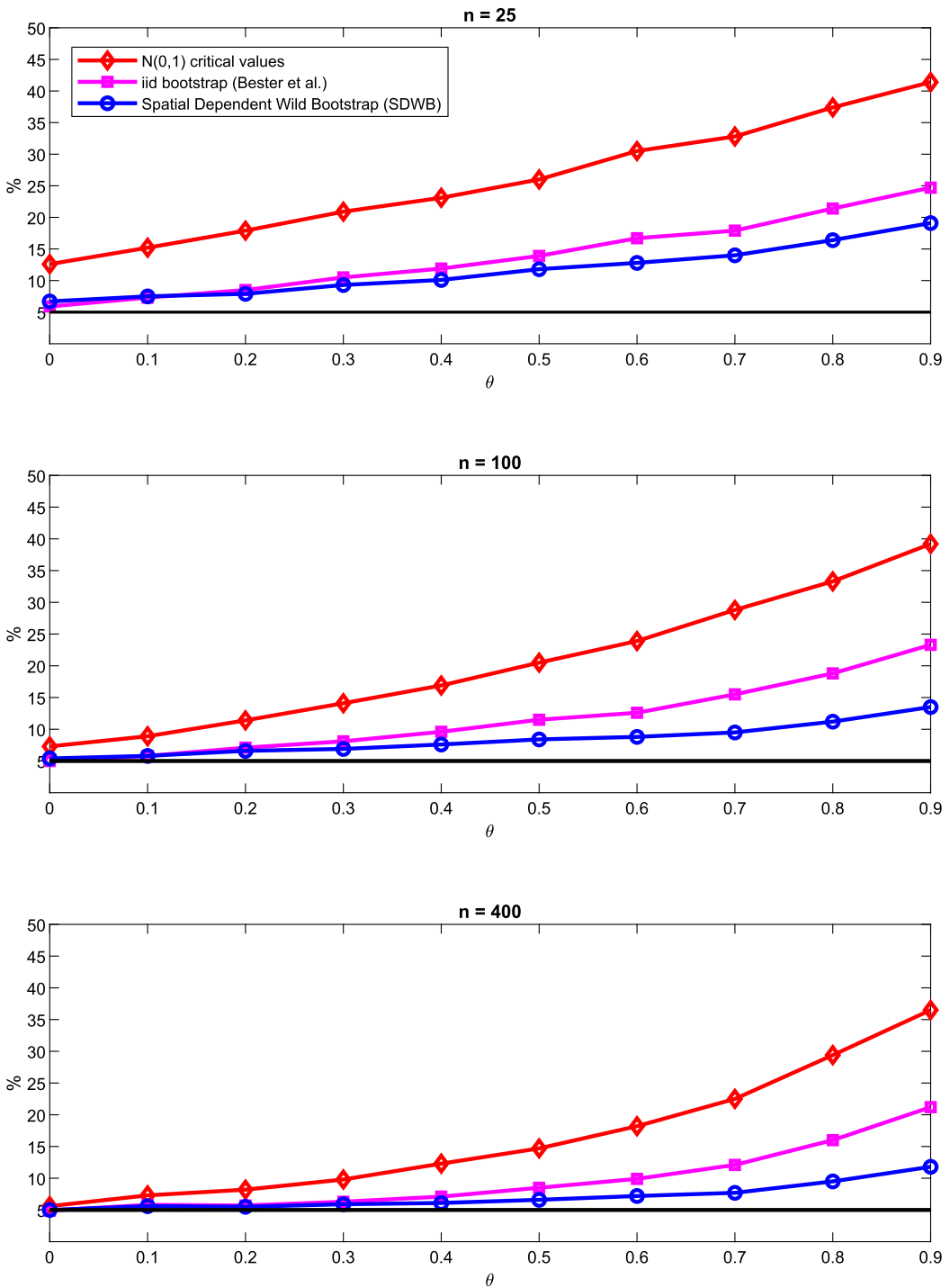
FIGURE 5. Rejection rate, max distance in DGP, Euclidean in sample.
