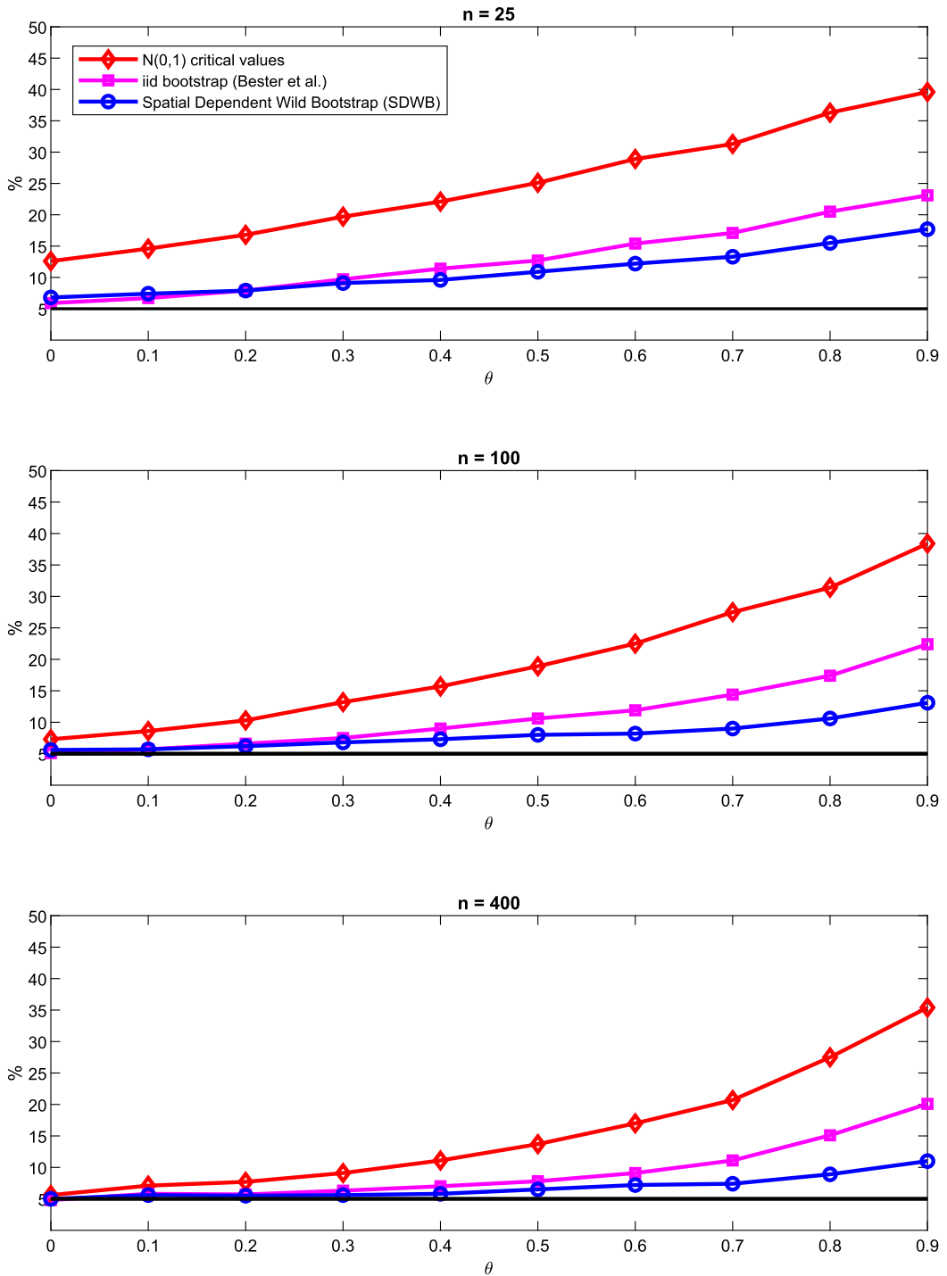
FIGURE 1. Rejection rate with no measurement error.
