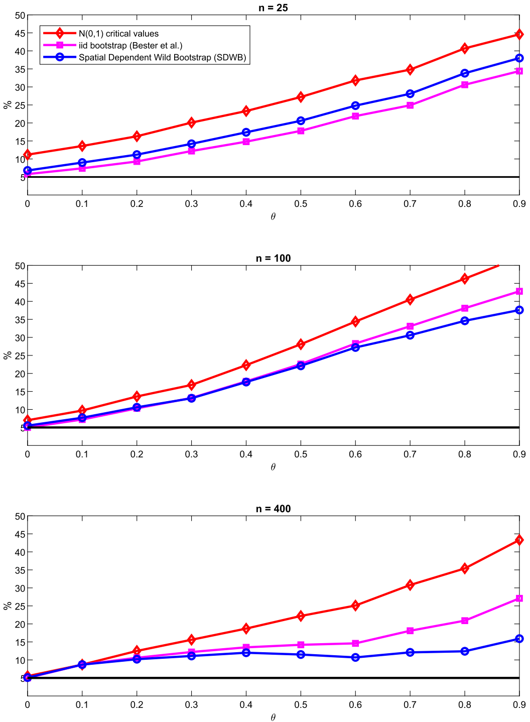
FIGURE 3. Rejection rate with N(0, 4) error in locations.
