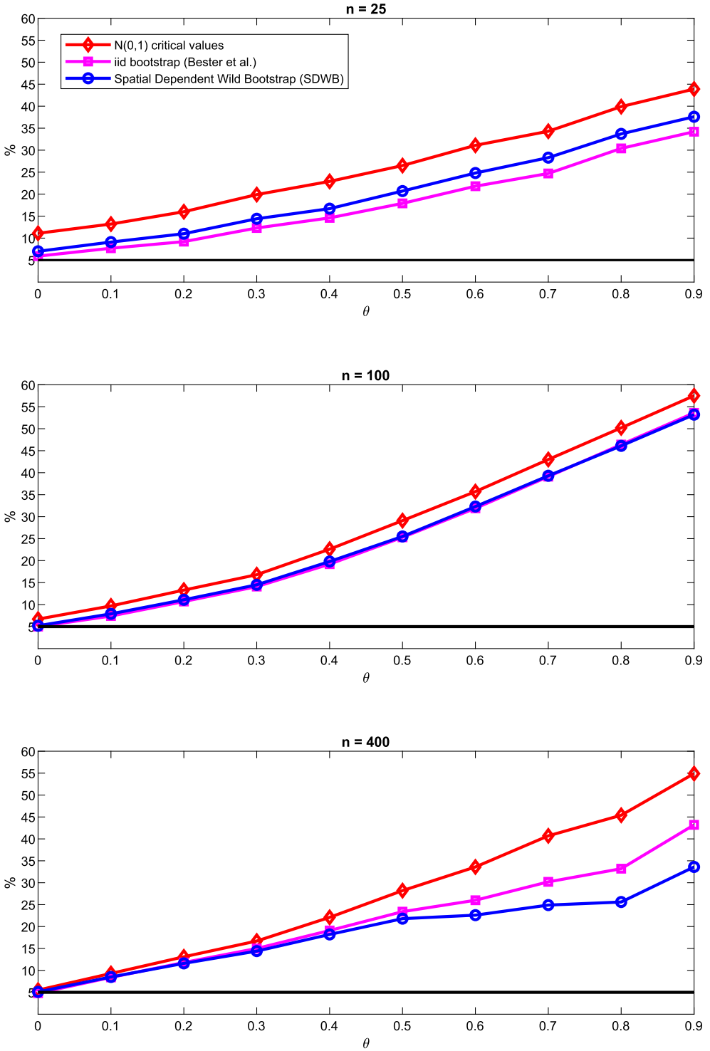
FIGURE 4. Rejection rate with N(0, 10) error in locations.
