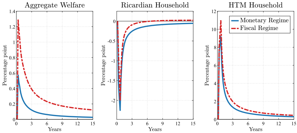
FIGURE 2. Short-Run Welfare Gains Comparison. Note: This figure presents the short-run welfare gains resulting from the redistribution, compared to the economy without transfer redistribution. The values are the difference in the welfare measures ( \mu_{t,k}^i ) between the transfer cases (under monetary and fiscal regimes) and the without-transfer case under the monetary regime as a function of time. Blue solid lines represent the short-run welfare gains under monetary regime and red dashed-dotted lines represent those under fiscal regime.
