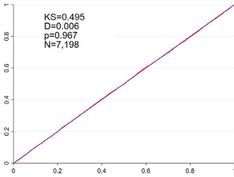
(a) An empirical c.d.f. of t -values
