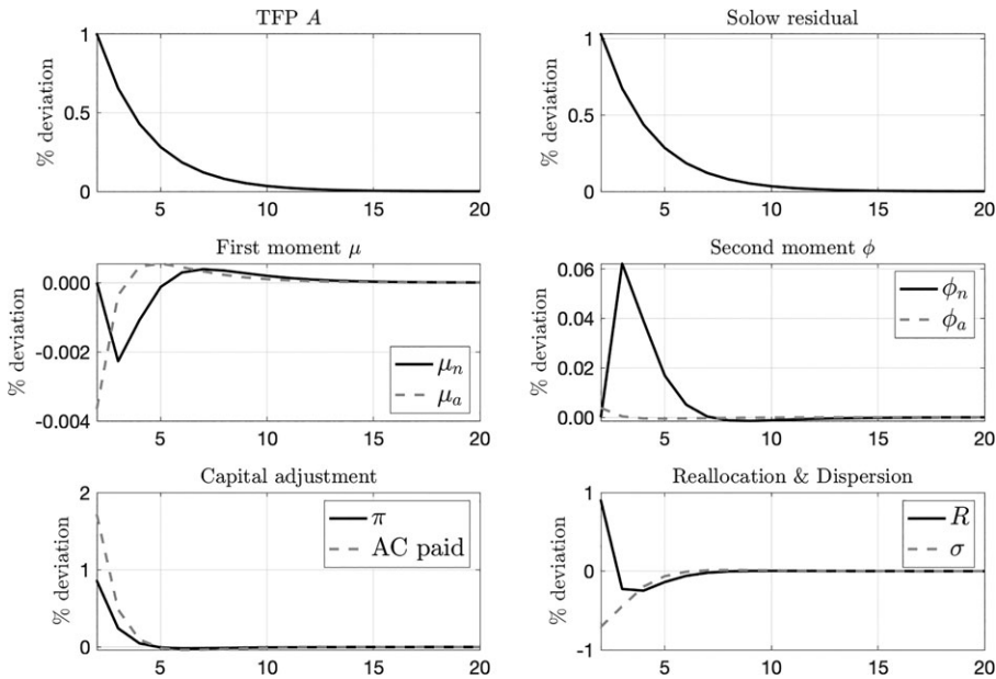
FIGURE 4. Impulse response functions: TFP shock.
