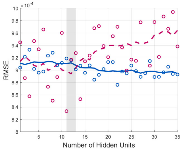
FIGURE 1. Root Mean Squared Error (RMSE) in function of the number of neurons in the hidden layer. Note: The figure shows the relation between the number of hidden units and neural network performance in the neoclassical growth model. Solid blue line—network performance on the training set. Dashed purple line—network performance on the validation set. Circles show network performance for a specific number of units. Lines represent the moving averages.
