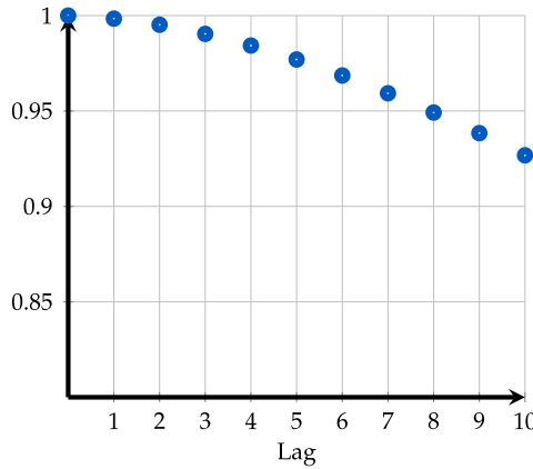
FIGURE 3. Autocorrelation function of the equilibrium bond sequence. Note: The figure shows the autocorrelation function of b_t^N . The numbers are obtained after simulating the model equilibrium dynamics for T = 5000 .
