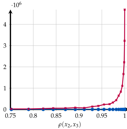
FIGURE 2. Mean squared prediction error with a neural network and a polynomial. Note: The figure shows the mean squared prediction error 1/n \sum_{t=1}^n [y_t - \mathbb{E}(\hat{y}_t)]^2 in function of the correlation between x_2 and x_3 . Blue line with circles—NN, purple line with crosses—polynomial regression.
