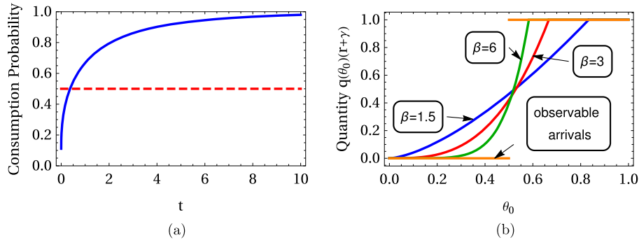
FIGURE 3. (a) Consumption probability over time: progressive (solid); dynamic (dashed). The initial valuation is uniformly distributed on [0, 1] , \beta = 1.5 , and \sigma = 1 . (b) Quantities assigned in progressive mechanism for: \beta = 1.5 , \beta = 3 , and \beta = 6 , observable arrival in horizontal lines. The initial valuation is uniformly distributed on [0, 1] .
