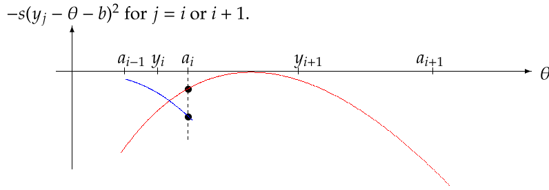
FIGURE 1. x_{i+1} < x_i + 4b .
