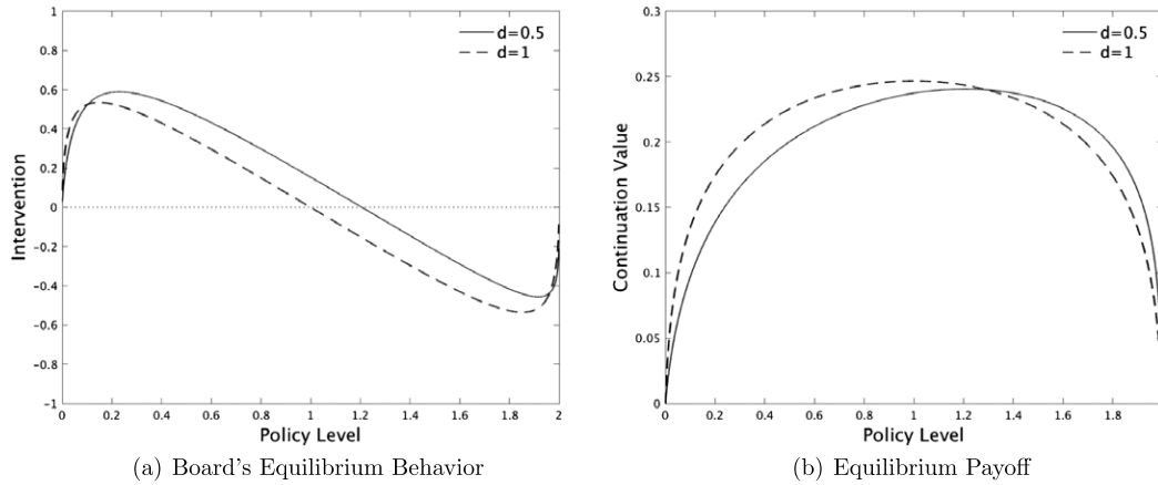
FIGURE 2. Parameters: \lambda = 0.5, \theta = 0.4, c = 1, r = 0.1 .
