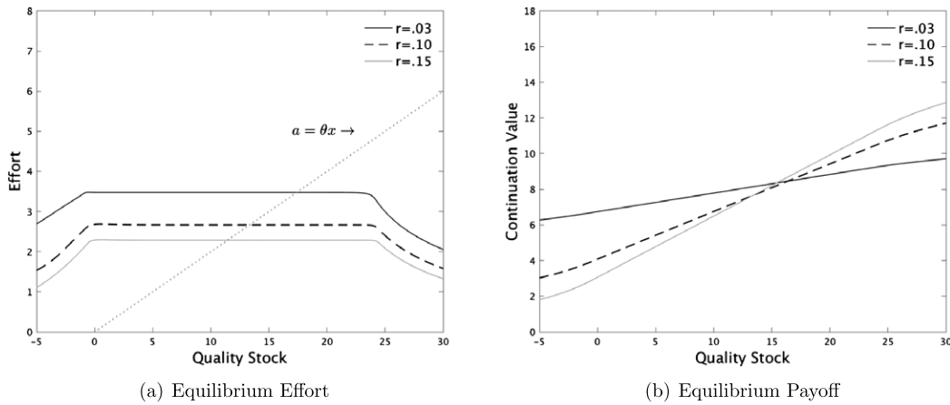
FIGURE 1. Parameters: \lambda = 0.8 , \bar{B} = 20 , \theta = 0.2 .
