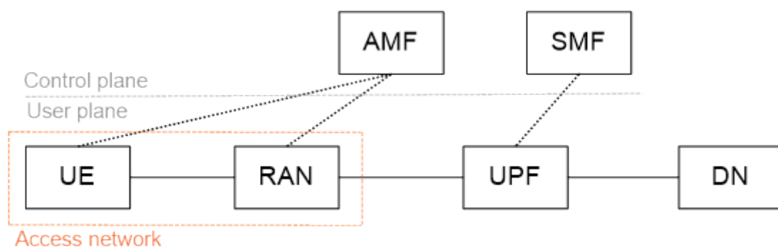
FIGURE 1: 5G network architecture.
