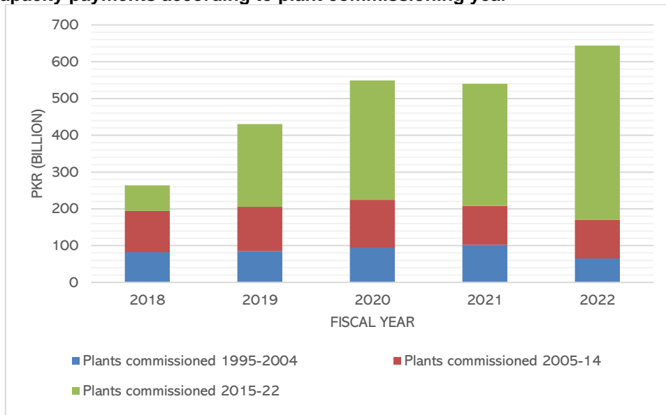
Figure 3: Capacity payments according to plant commissioning year
