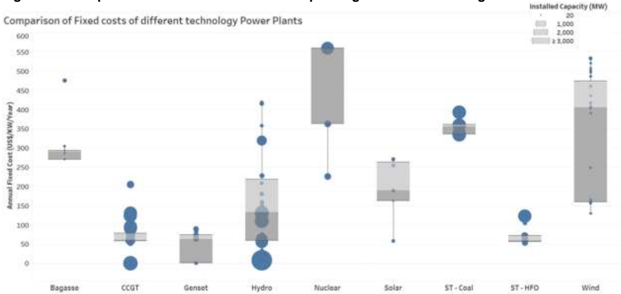
Figure 16: Comparison of fixed costs of different power generation technologies
