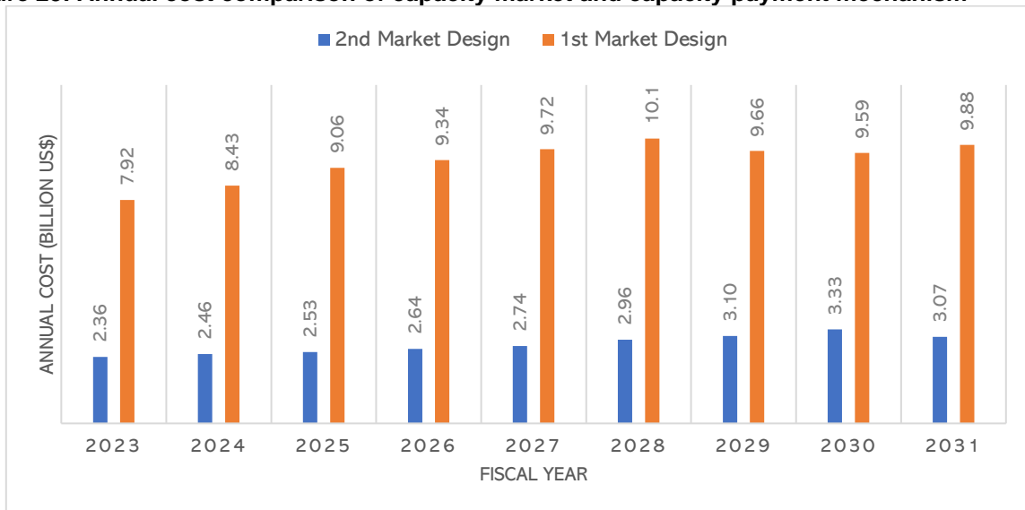
Figure 25: Annual cost comparison of capacity market and capacity payment mechanism
