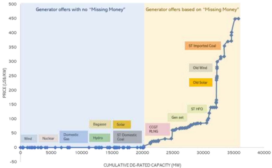
Figure 22: Capacity supply curve for FY 2023
