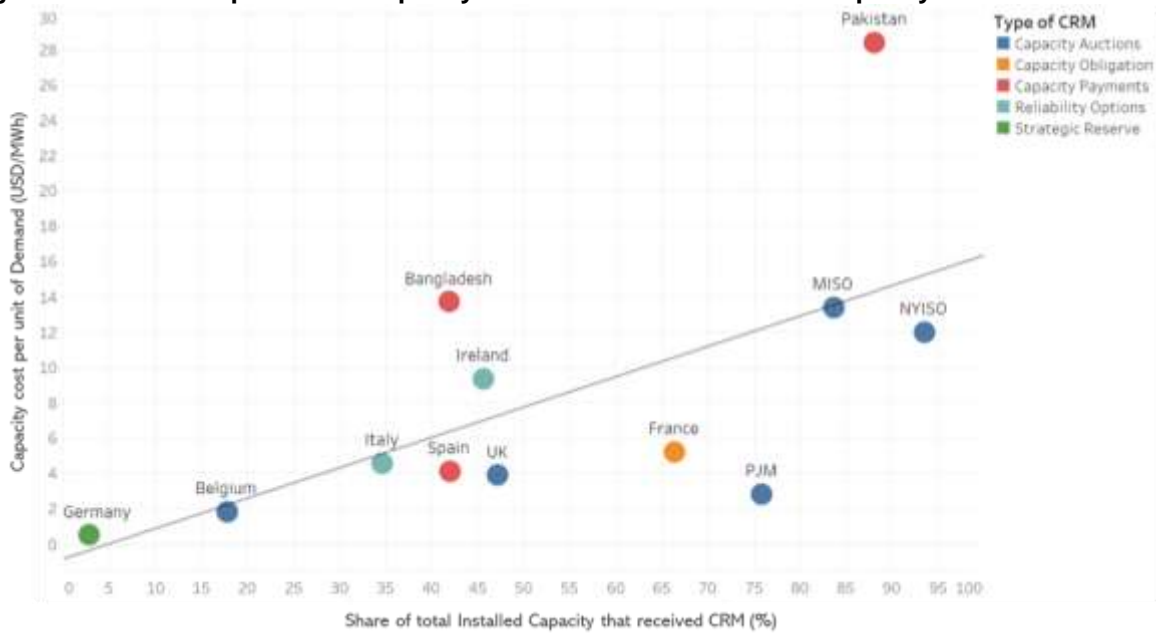
Figure 8: Relationship between capacity cost and share of installed capacity that received CRM
