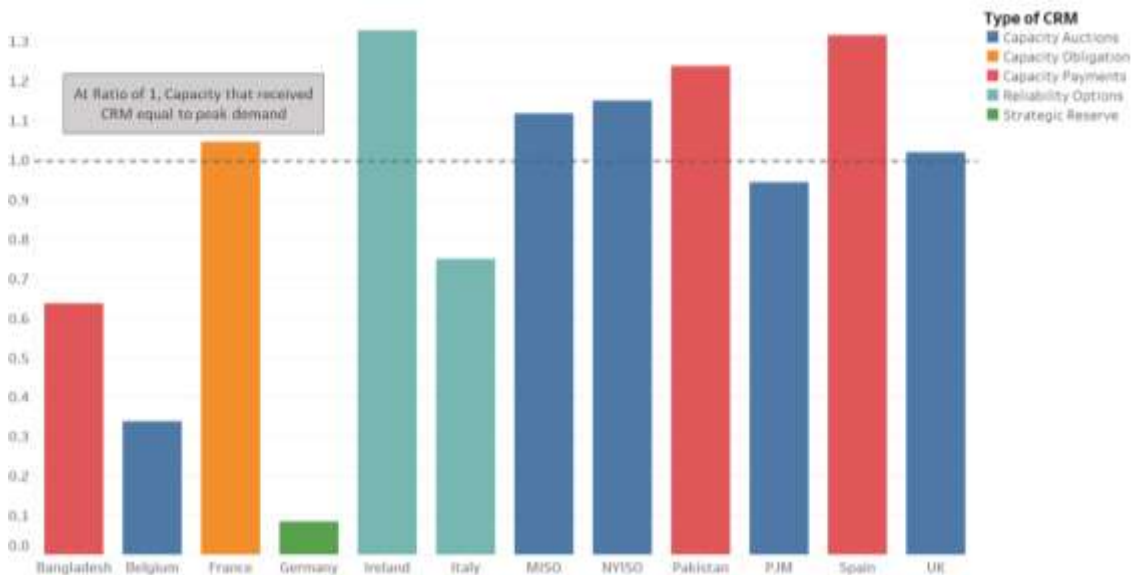
Figure 9: Ratio between peak load and capacity that received CRM
