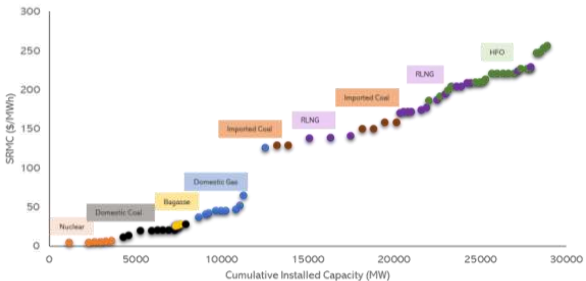
Figure 15: Short-run marginal cost of thermal, nuclear, and bagasse power plants
