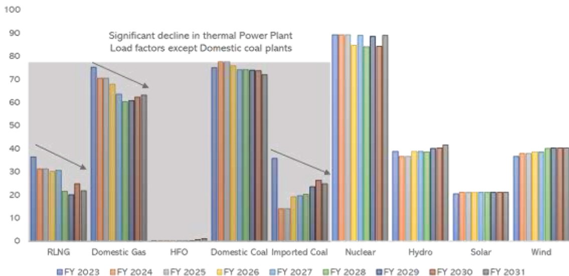
Figure 21: Weighted Average Load Factor of thermal Power Plants from FY 2023 to FY 2031
