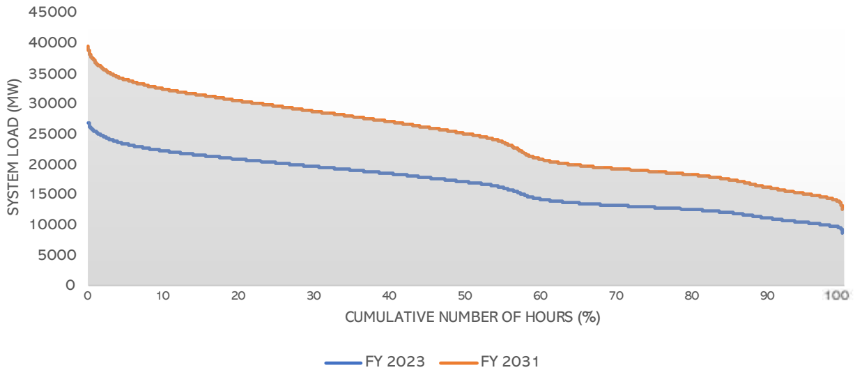
Figure 14: Load duration curve for national grid system, FY 2023 and 2031
