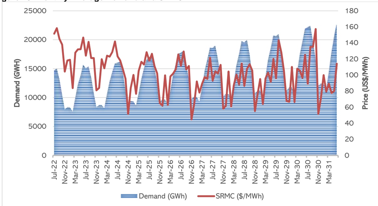
Figure 19: Monthly Average Demand and SRMC
