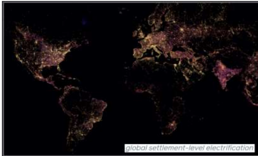
Figure 17: Global settlement level electrification 60
