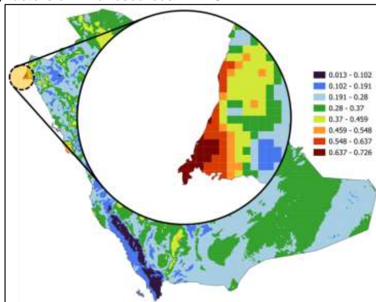
Figure 8: Capacity factors of wind resources in NEOM
