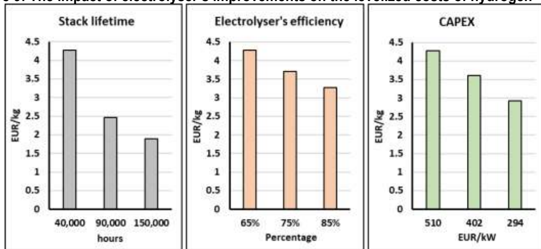
Figure 9: The impact of electrolyser's improvements on the levelized costs of hydrogen
