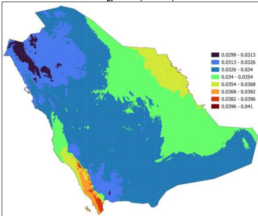
Figure A8: Levelized costs of solar energy in KSA (EUR/kWh)
