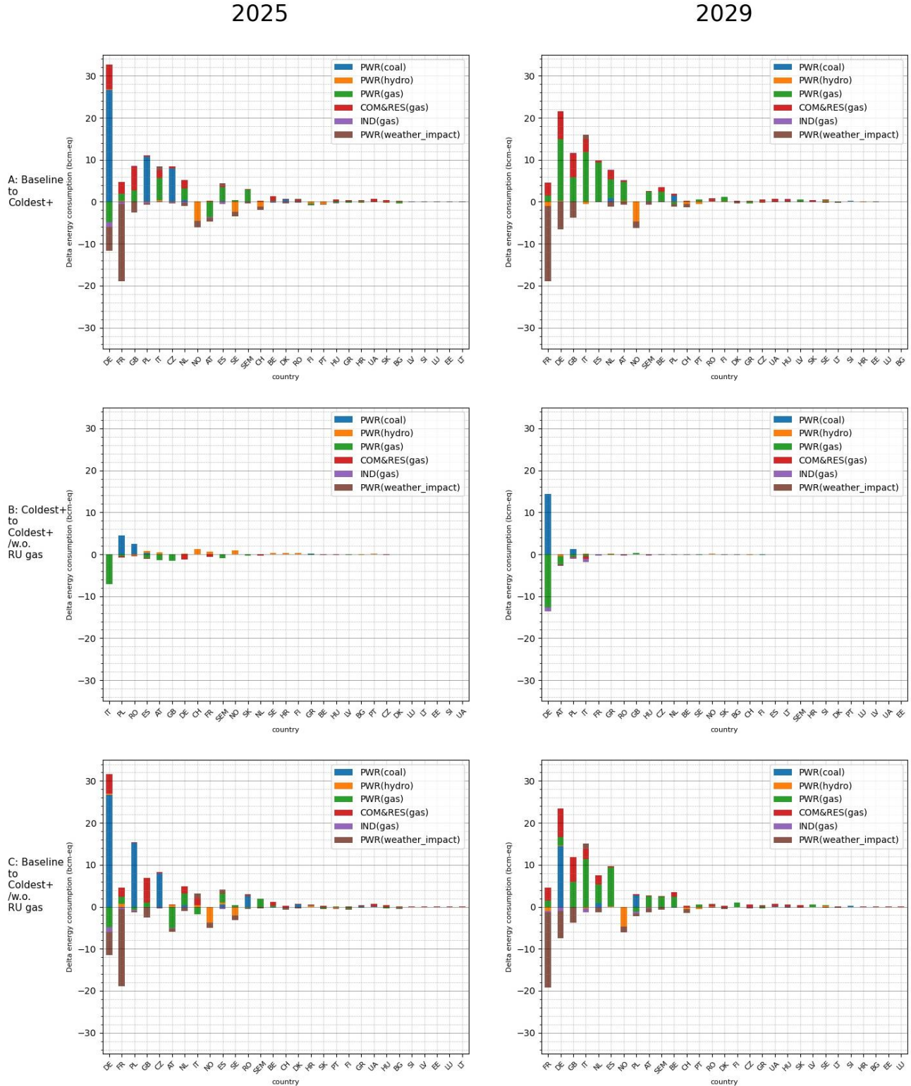
Figure 11: Extreme weather under the baseline (A), the impact of Russian gas phase-out (B), and total changes in electricity and gas consumption (C)
