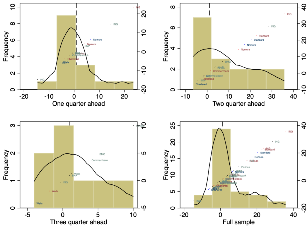
Figure 1: Coefficients of individual forecaster and currency level least squares regressions. Color blue: UK. Color red: Euro. Color Black: others.
