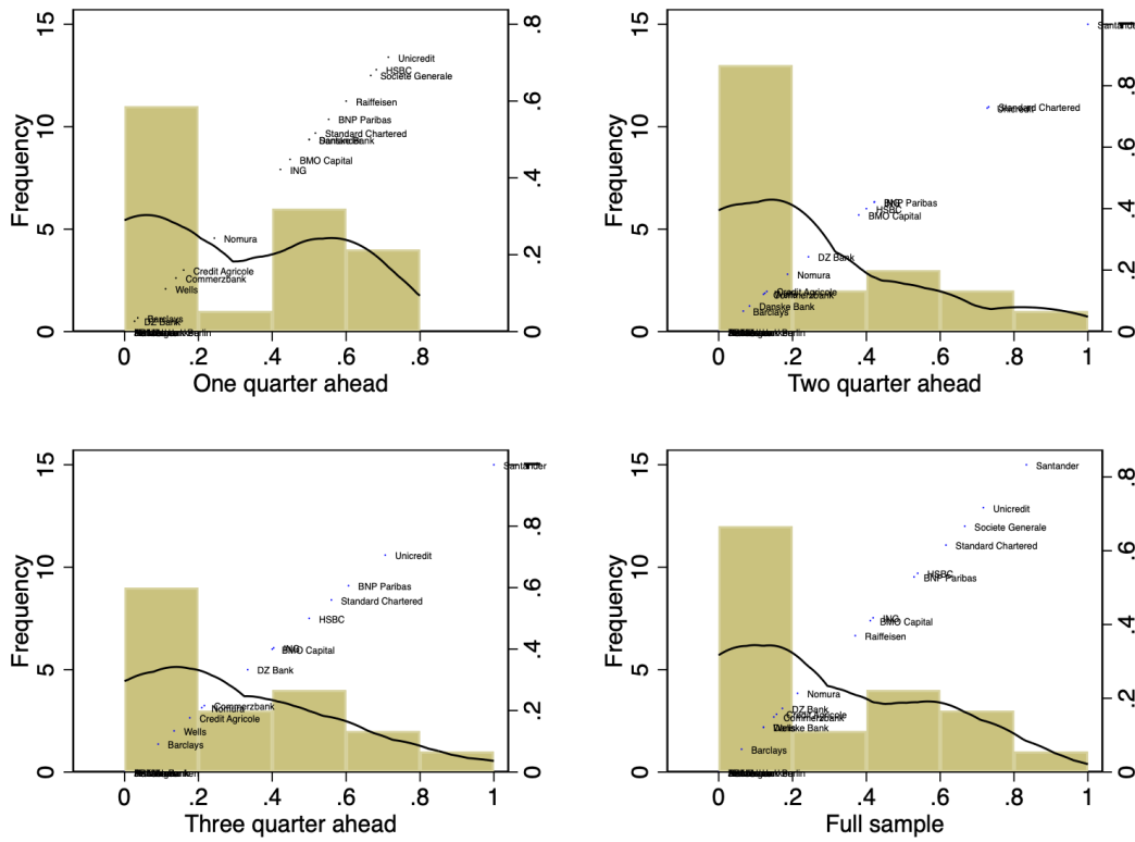
Figure 2: Directional Alignment With UIP
