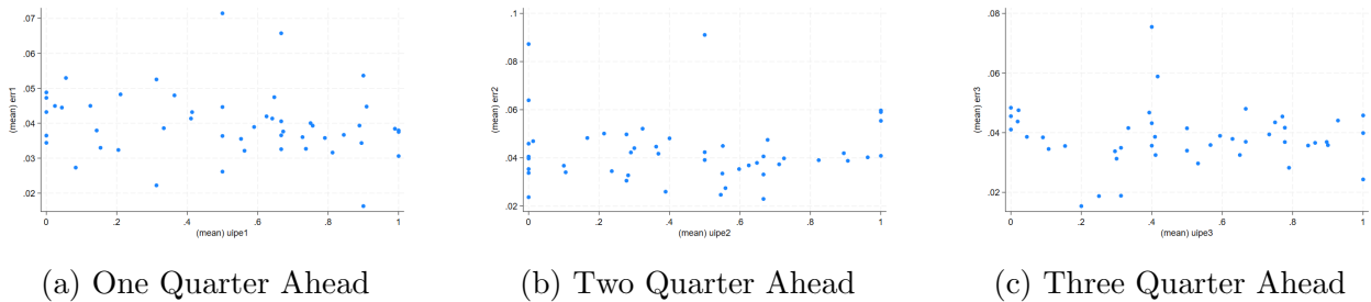
Figure 3: Are Forecasts that Match the UIP Direction Better?
