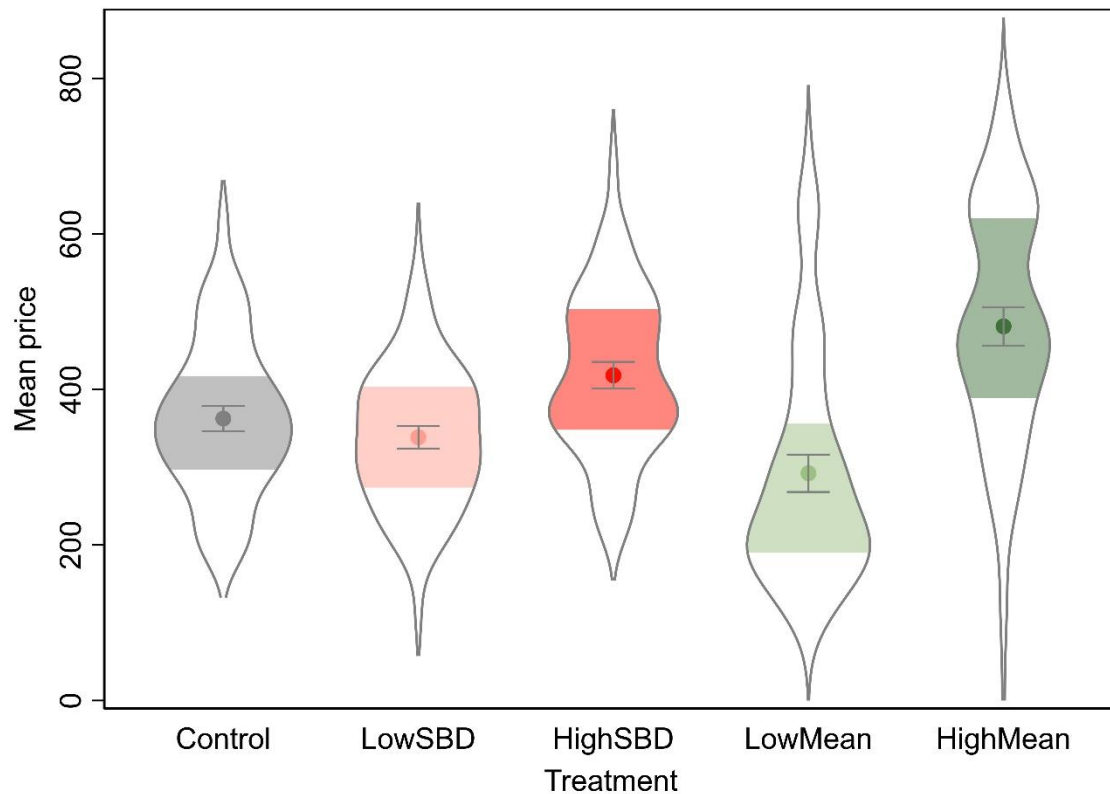
Figure 2. Distributions of Estimated Mean Hotel Prices by Treatment Group. Notes: In the LowMean and HighMean treatments, beliefs of the mean hotel price are directly stated by participants and in Control, LowSBD and HighSBD means are inferred from participants' SBDs. The central marker within each shaded area indicates the mean estimate, with bars representing the corresponding 95% confidence intervals. The shaded/coloured areas depict the interquartile ranges.
