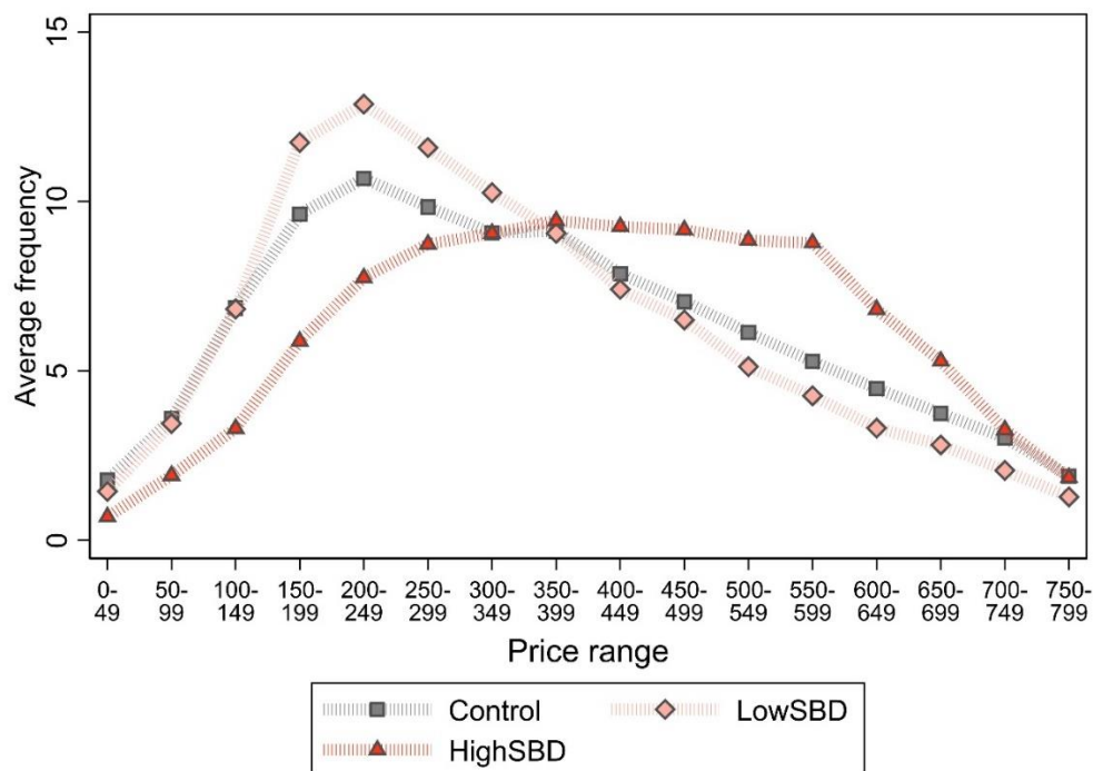
Figure 5. Average stated frequencies for each price interval in the SBD elicitation by treatment.
