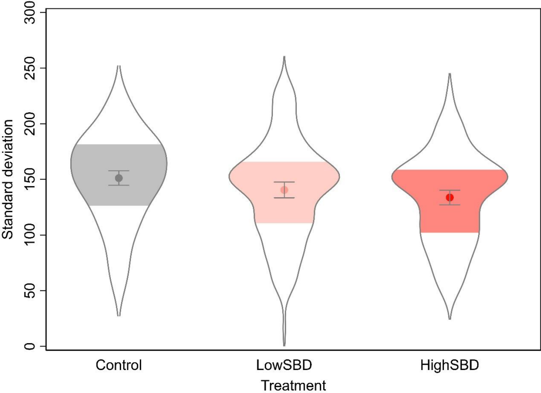
Figure 4. Average mean and standard deviation in SBD treatments. Notes: The central marker within each shaded area indicates the mean estimate, with bars representing the corresponding 95% confidence intervals. The shaded/coloured areas depict the interquartile ranges.
