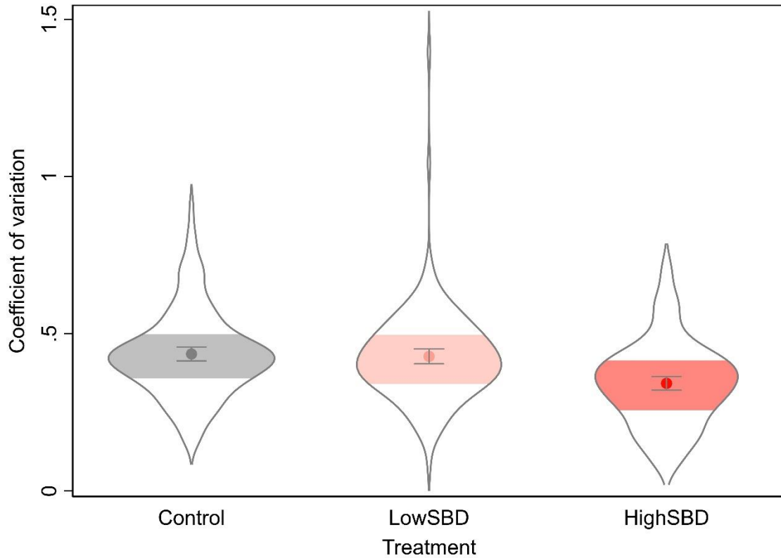
Figure 3. Average coefficient of variation in SBD treatments. Notes: The central marker within each shaded area indicates the mean estimate, with bars representing the corresponding 95% confidence intervals. The shaded/coloured areas depict the interquartile ranges.
