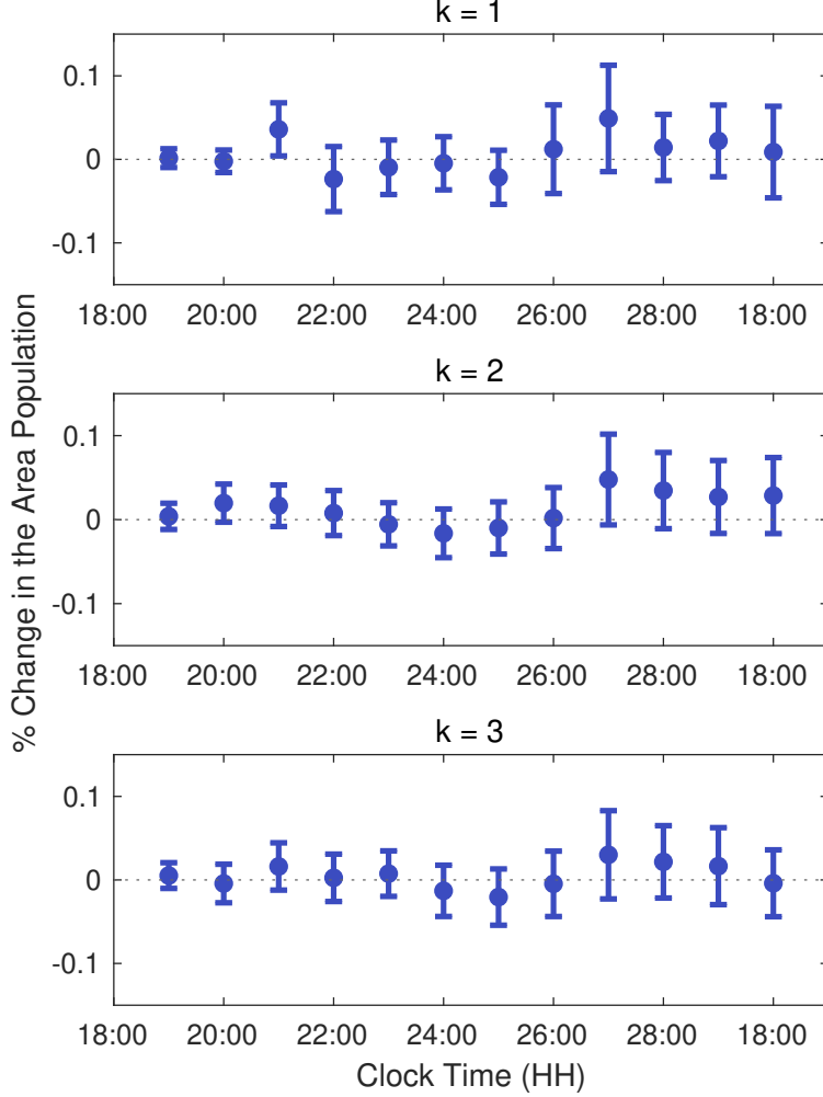
Figure 8: Placebo Test
