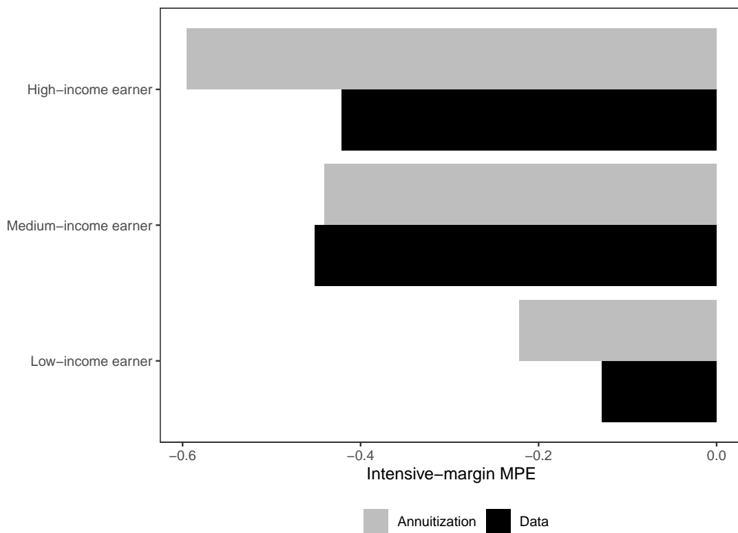
Figure A.1: Comparison between annuitization method and observed intertemporal behavior
