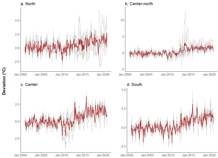
Figure 5. Temperature and precipitation deviations from the climate normal, 2001-2020 a) Temperature
