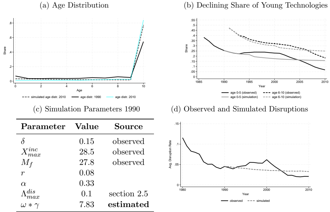
Figure 6: Counterfactual Simulation
