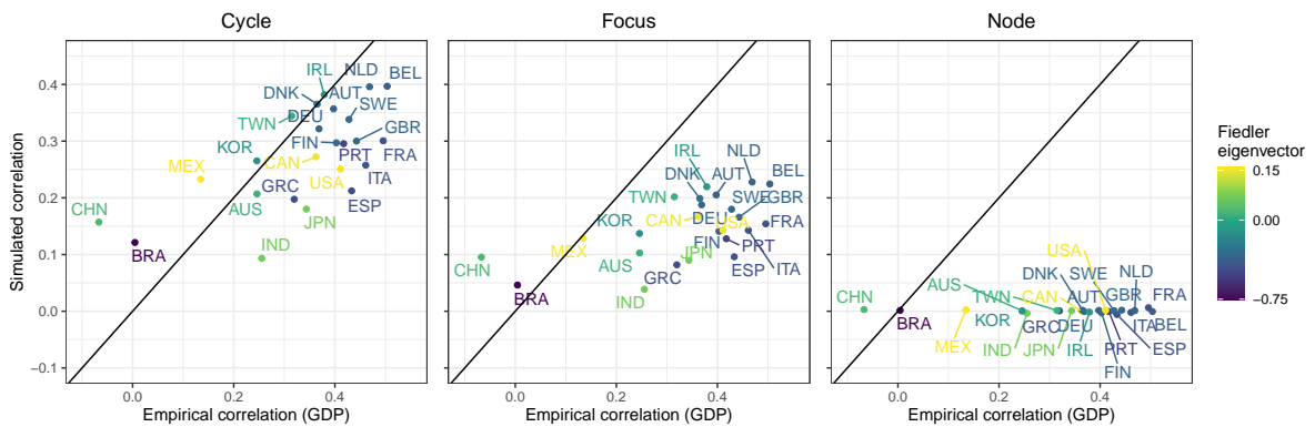
Figure 11: Mean Pearson correlation across the decision variable y of one country and the decision variables of all the other countries in our sample, in the model and in the data, averaged across 100 replications. The color code follows the position of the countries in the interaction network as exemplified by the Fiedler eigenvector, as in Figure 7. The identity line is plotted for reference.
