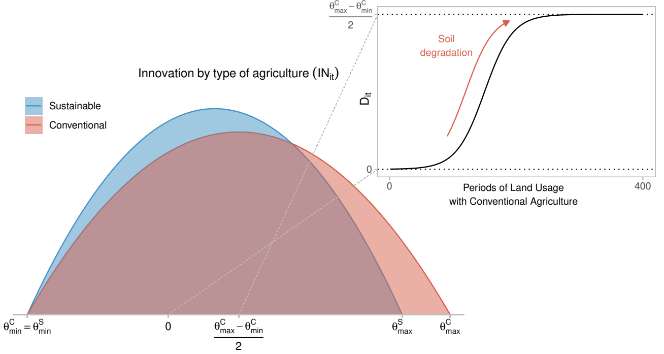
Figure 1: Soil productivity dynamics in different agricultural regimes.
