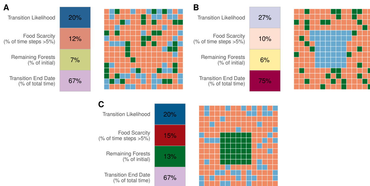
Figure 10: Heat-maps for different initial spatial scenarios.
