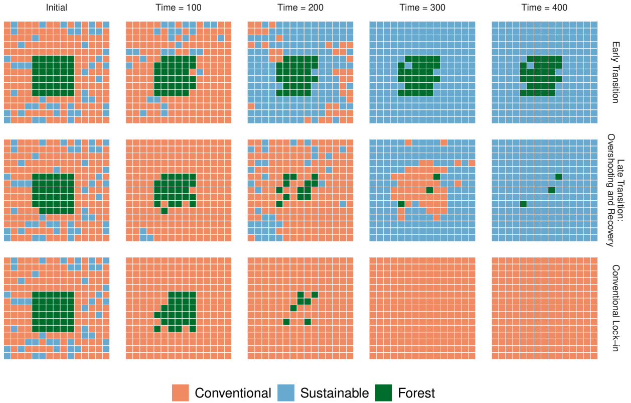
Figure 4: Spatial grid view of transition, overshooting and lock-in scenarios in the model.
