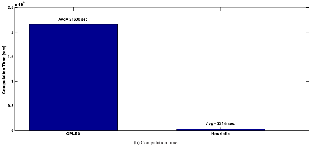
Figure 4: Gap and computation time produced by heuristic for large data sets
