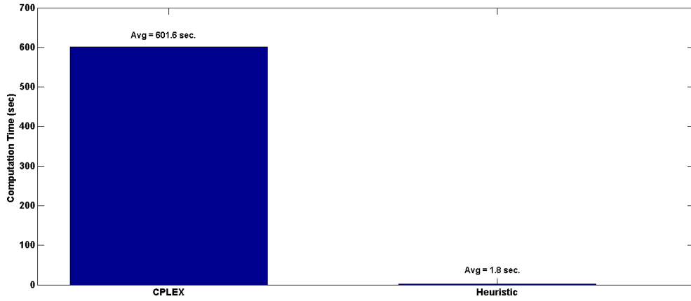
(b) Computation time
