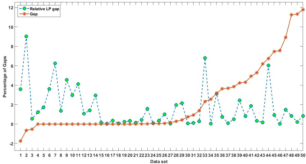
Figure 3: Gaps and Relative LP Gaps
