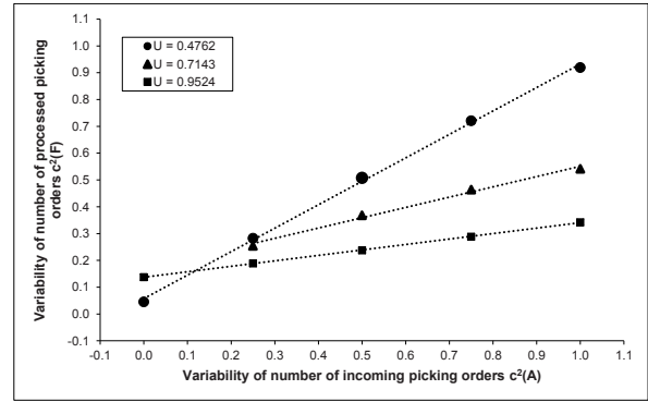
Fig.8: Impact of variability of incoming picking orders c^2(A) and traffic intensity U on variability of processed picking orders c^2(F) (Note: There is no value of c^2(F) for scenario (E(A) = 1.5, c^2(A) = 0.0) , since the value range of A is integer.)
