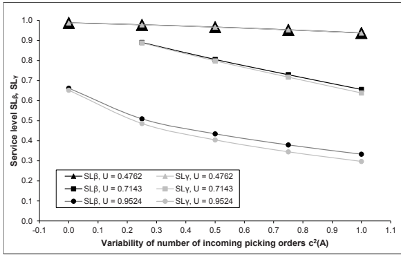
Fig.7: Impact of variability of incoming picking orders c^2(A) and traffic intensity U on \beta -service level SL_\beta and \gamma -service level SL_\gamma (Note: There is no value of SL_\beta , SL_\gamma for scenario (E(A) = 1.5, c^2(A) = 0.0) , since the value range of A is integer.)
