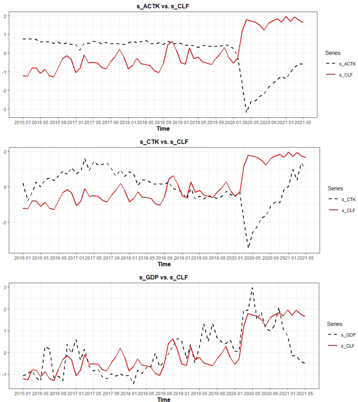
Figure 3: The standardized time series plot comparing s_CLF and s_ACTK, s_CTK, s_GDP
