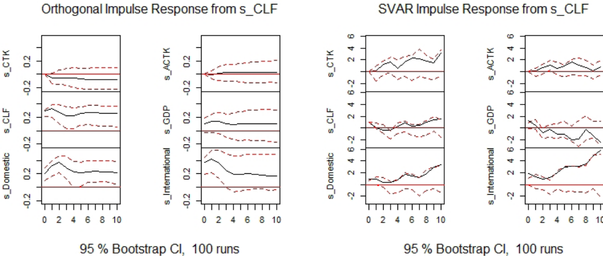
Figure 5: s_CLF impulse response
