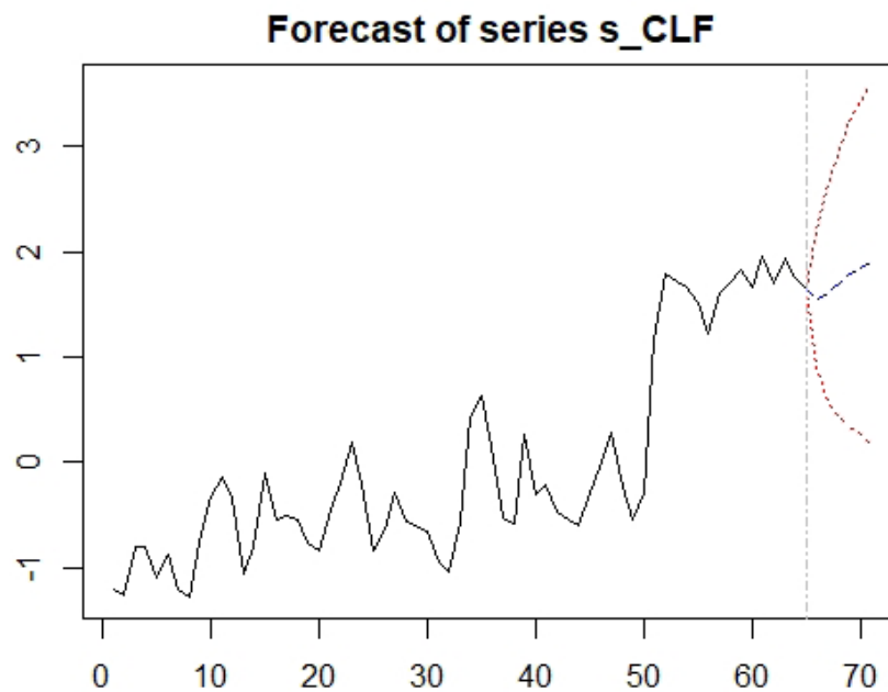
Figure 7: Forecasting of s_CLF
