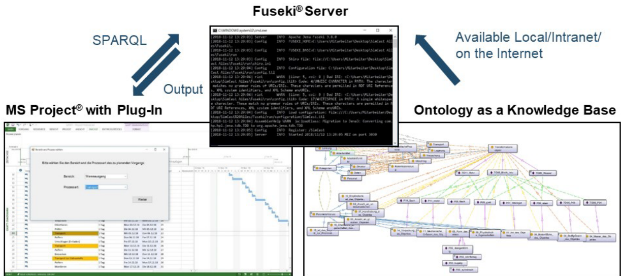
Figure 12: Access to the knowledge structure
