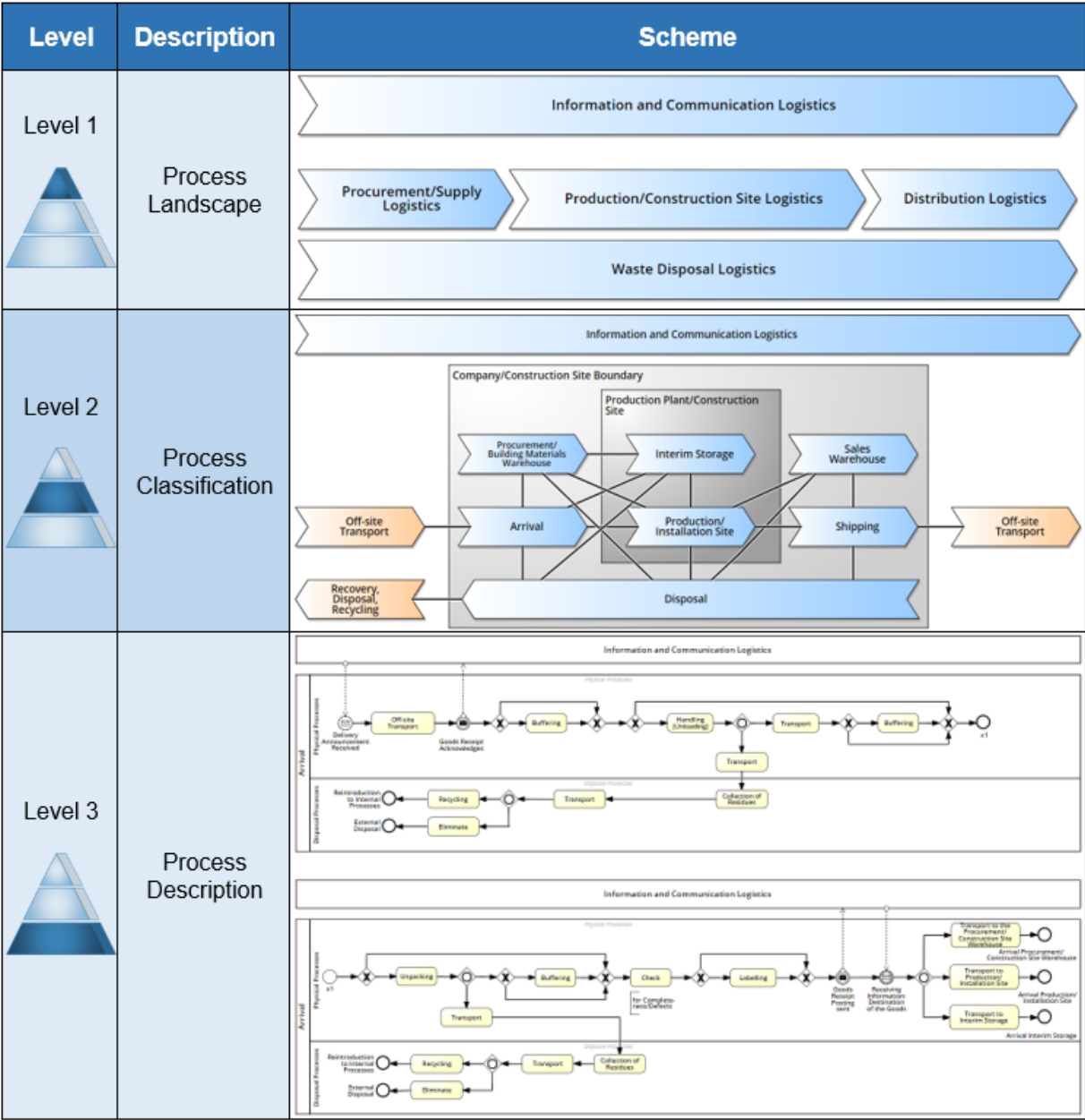
Figure 3: Levels of detail of the reference model (own representation based on the SCOR model)
