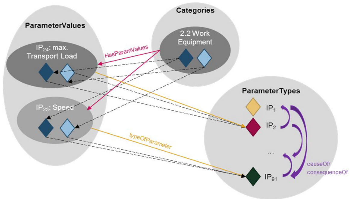
Figure 8: Ontology concept III
