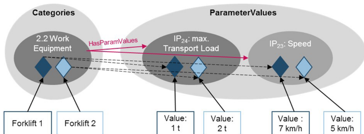
Figure 7: Ontology concept II
