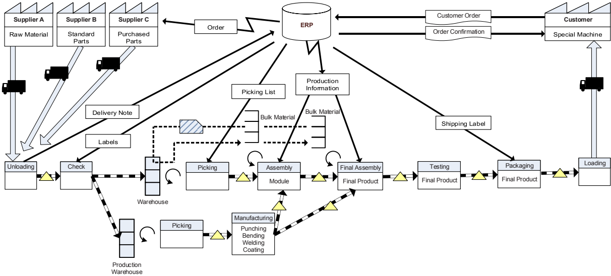
Figure 13: Company specific value stream (exemplary presentation)
