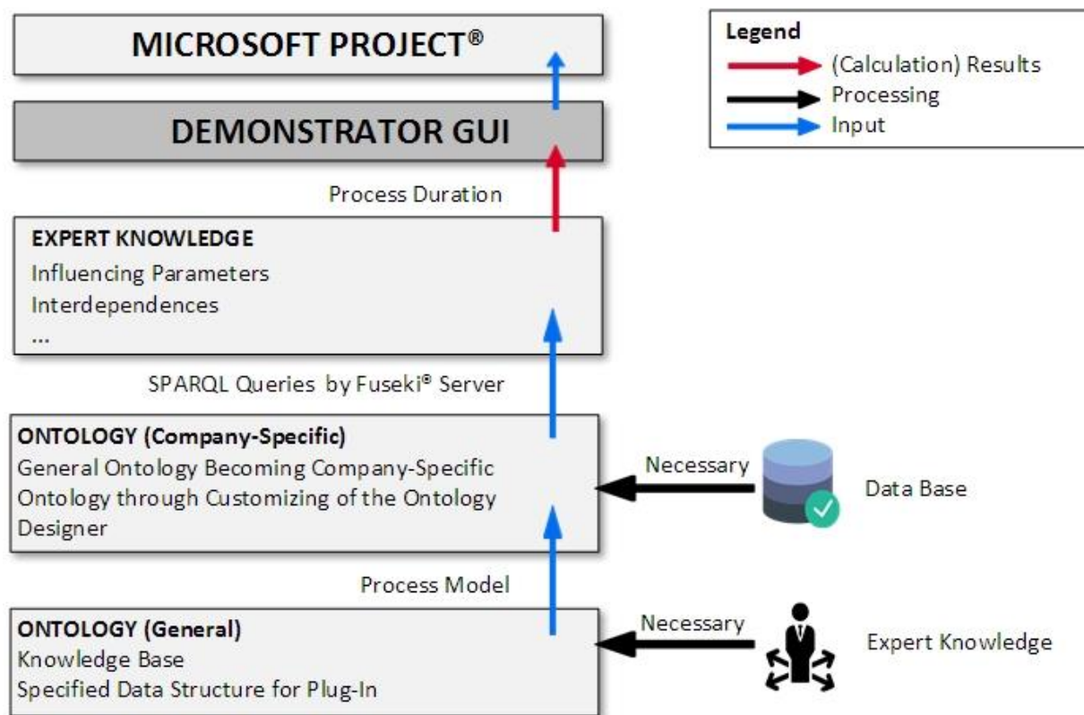
Figure 21: System architecture of the demonstrator
