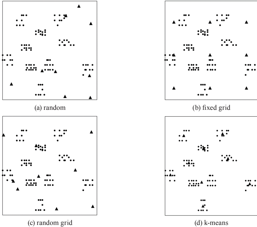
Fig. 1: Different strategies for generating locations of potential locker box stations. Circles represent customer nodes and triangles represent locker box locations.
