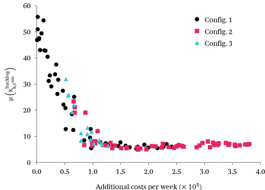
Fig. 14: Comparison of the Configurations 1-3 regarding additional costs and average tardiness
