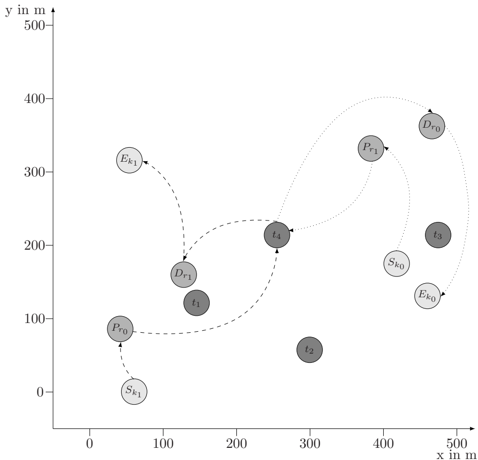
Figure 4: Solved problem instance considering a transport load transfer (note: arcs are just for visualization purpose)
