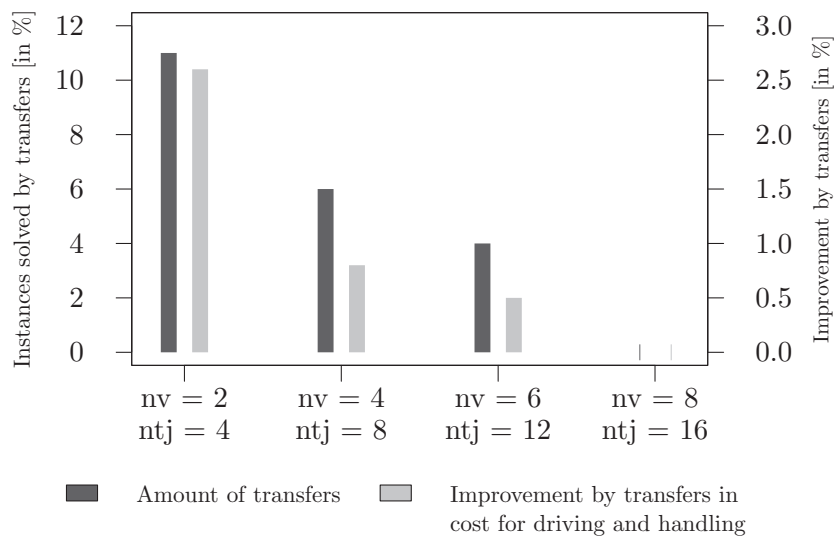
Figure 5: Percentage of test instances solved with at least one transfer operation and average improvement compared to the solution neglecting transfers (from ALNS-wot) concerning problem size for a time-limit of 30 s
