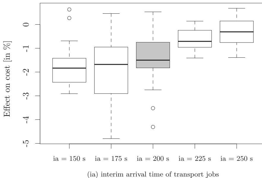
Figure 9: Effect on different throughput levels on the cost of transport execution; whiskers limits are set to 1.5 times the interquartile range from lower to upper quartile
