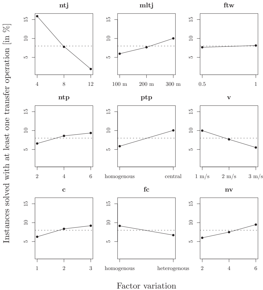
Figure 7: The influence of basic system characteristics to the percentage of solutions solved by transport load transfers
