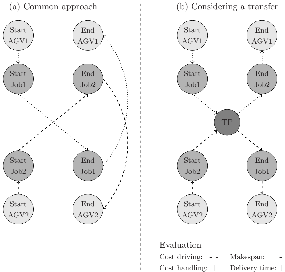
Figure 1: Comparison of a task assignment neglecting (left) and considering (right) a transport load transfer
