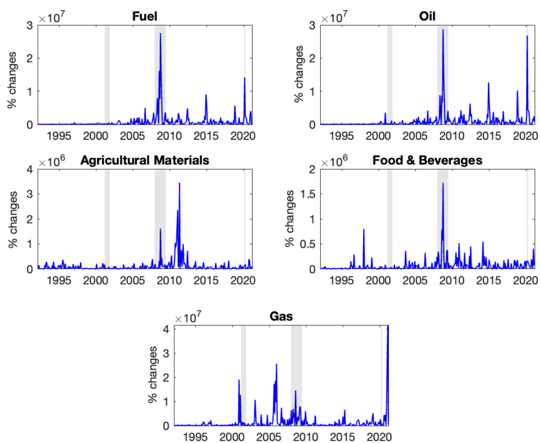
Figure 2: Commodity prices volatility measured as the square monthly percentage changes in the commodity reported in the title
