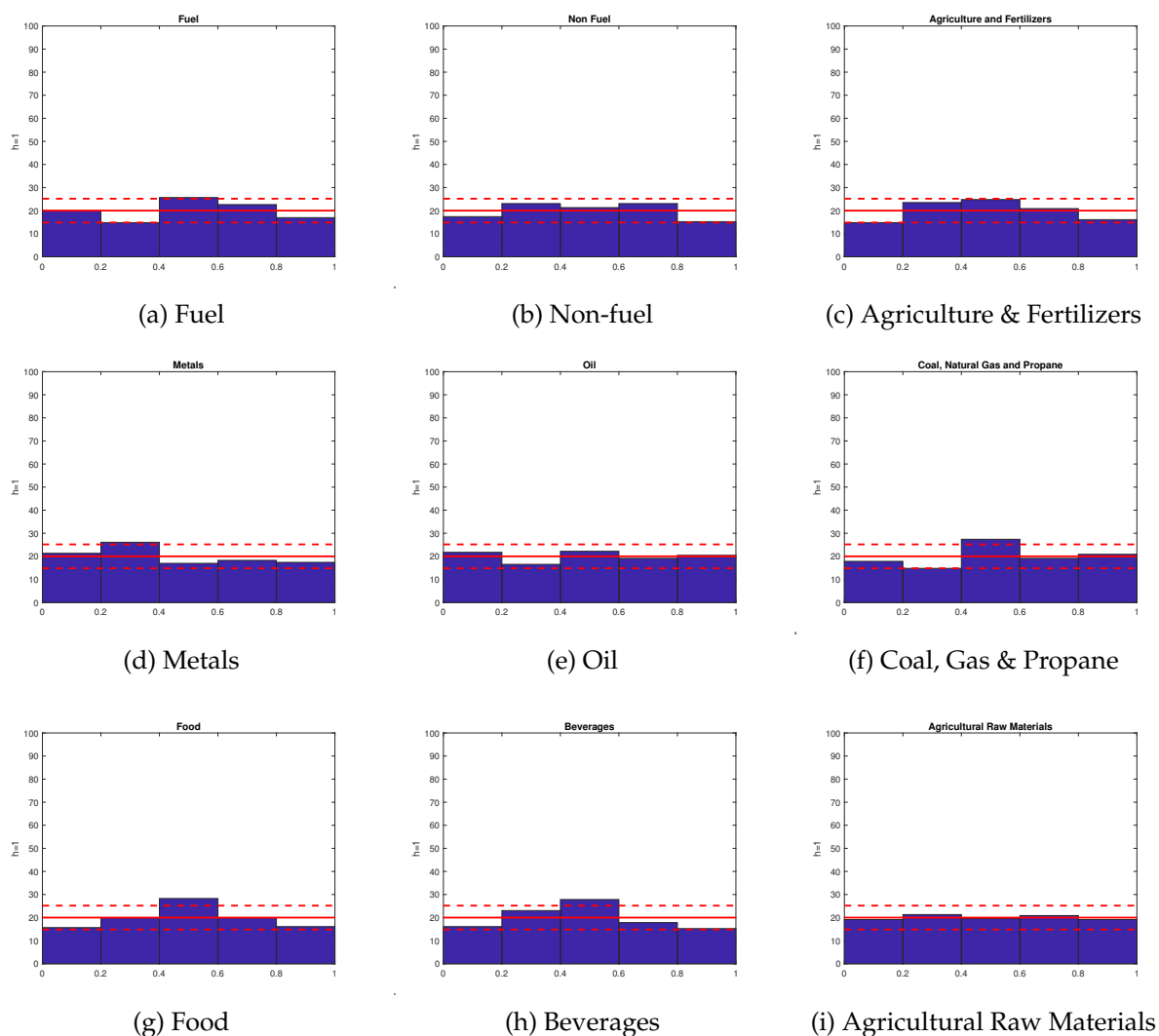
Figure A.5: Probability density functions of the PITs for the tvp model for one-month ahead forecasts of the nine remaining commodity indices. The dashed lines are 95% confidence intervals, constructed using a normal approximation to a binomial distribution, as per Diebold et al. (1998)
