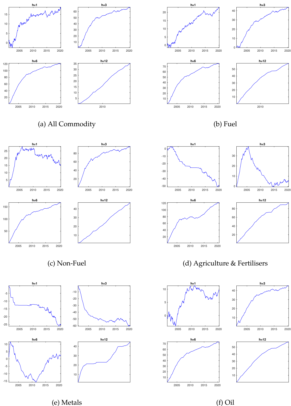
Figure 8: Cumulative differences in log-predictive likelihood of the model allowing for both time-varying slope and volatility (tvp) relative to the model that only allows for time-varying slope. Increases in the statistic denote dates in which tvp outperforms the alternative.
