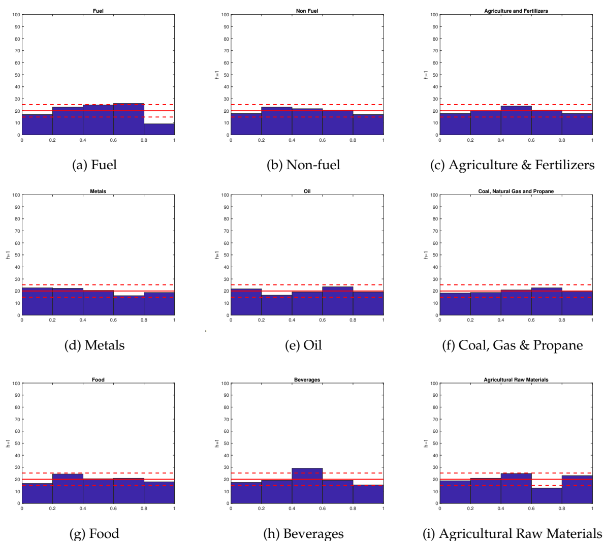
Figure A.6: Probability density functions of the PITs for the tvpBlocks model for one-month ahead forecasts of the nine remaining commodity indices. The dashed lines are 95% confidence intervals, constructed using a normal approximation to a binomial distribution, as per Diebold et al. (1998)
