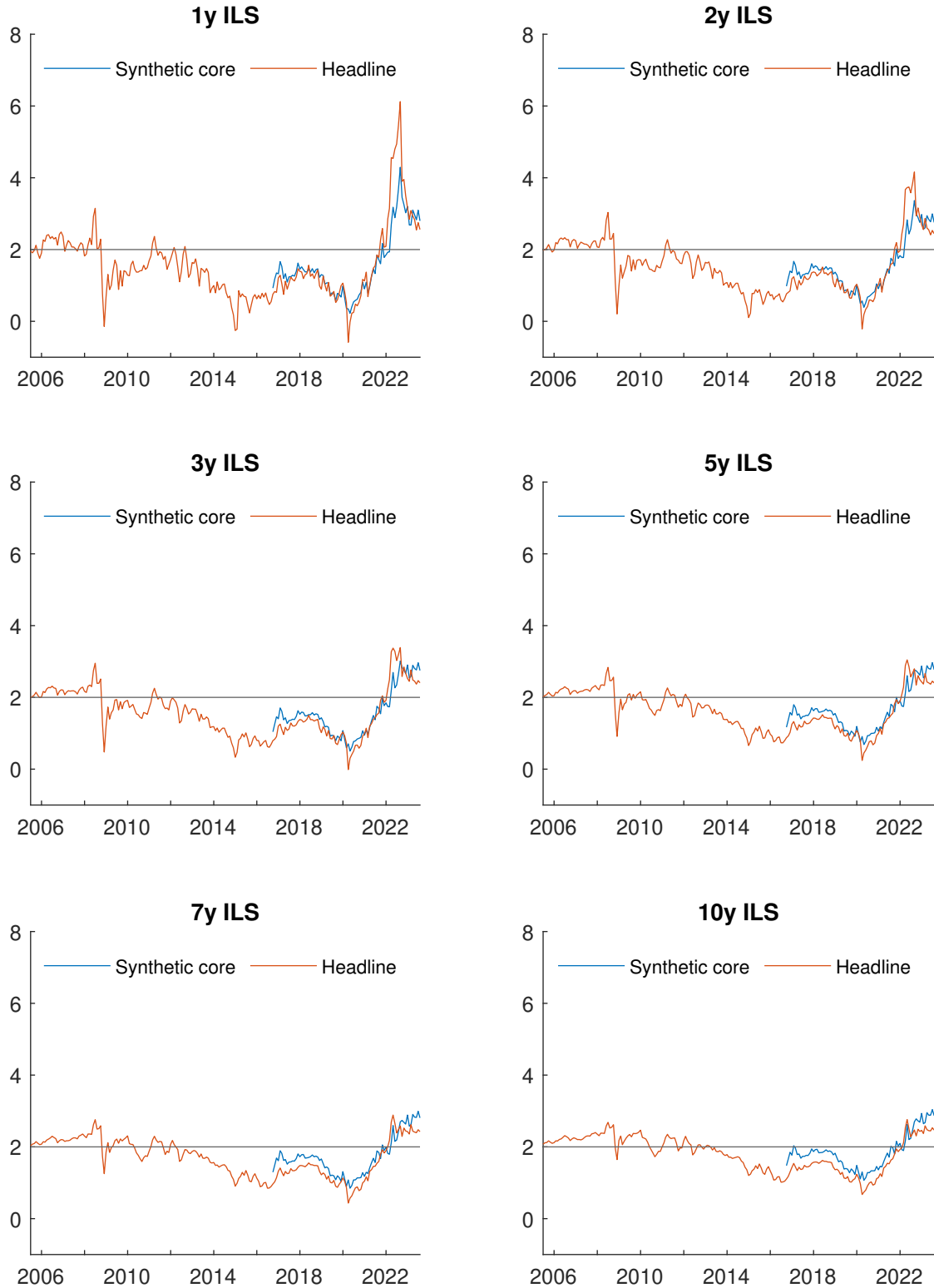
Figure 6: Model-implied core ILS rates
