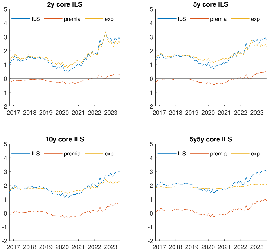
Figure 7: Decomposition of synthetic core ILS rates
